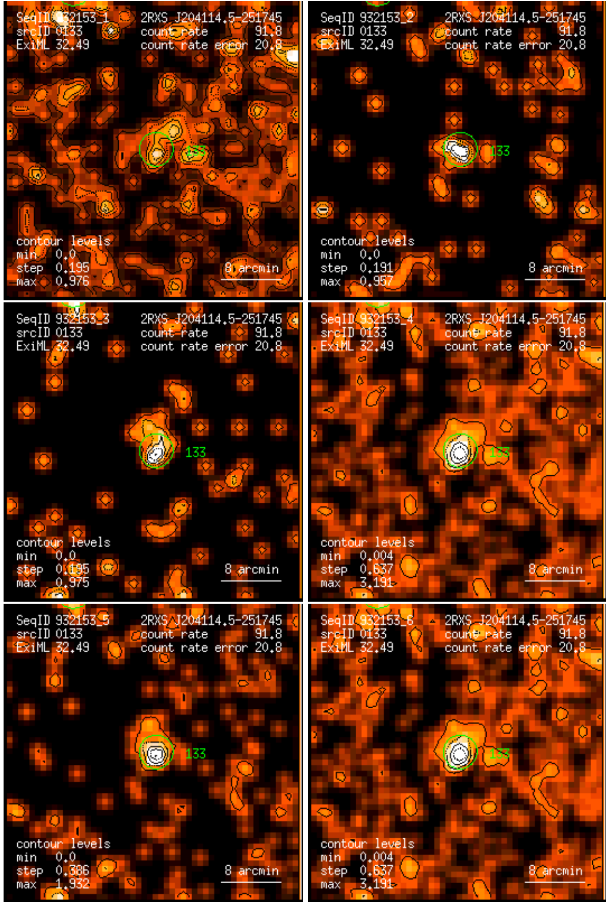
Figure 133: RASS 932153: detection 0133: band rate images, Gaussian filter: (1) PSPC channels 11 – 41, (2) 52 – 90, (3) 91 – 201, (4) 11 – 235, (5) 52 – 201, (6) 11 – 201. Broad band rates in counts/ks. Band rate contour levels in counts/ks/arcmin 2 .
