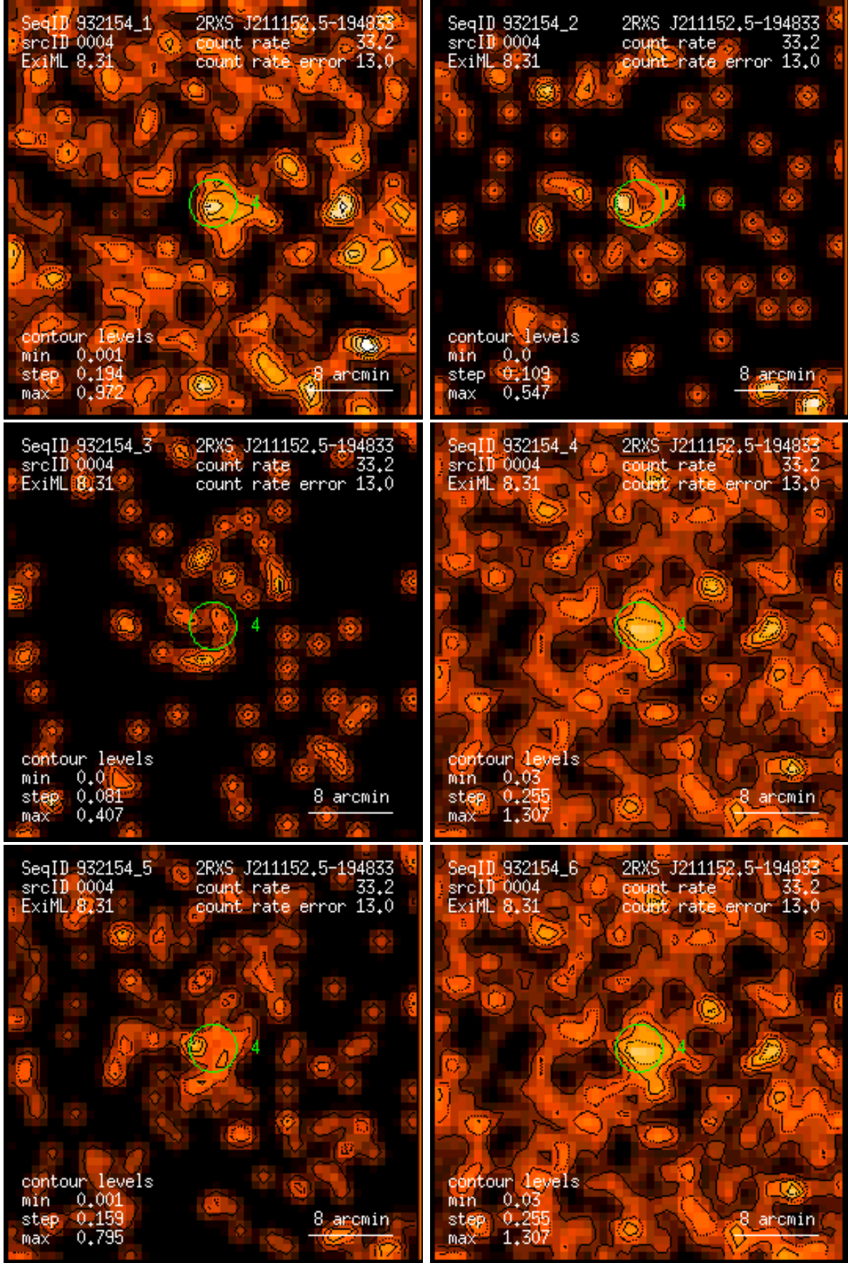
Figure 4: RASS 932154: detection 0004: band rate images, Gaussian filter: (1) PSPC channels 11 – 41, (2) 52 – 90, (3) 91 – 201, (4) 11 – 235, (5) 52 – 201, (6) 11 – 201. Broad band rates in counts/ks. Band rate contour levels in counts/ks/arcmin 2 .
