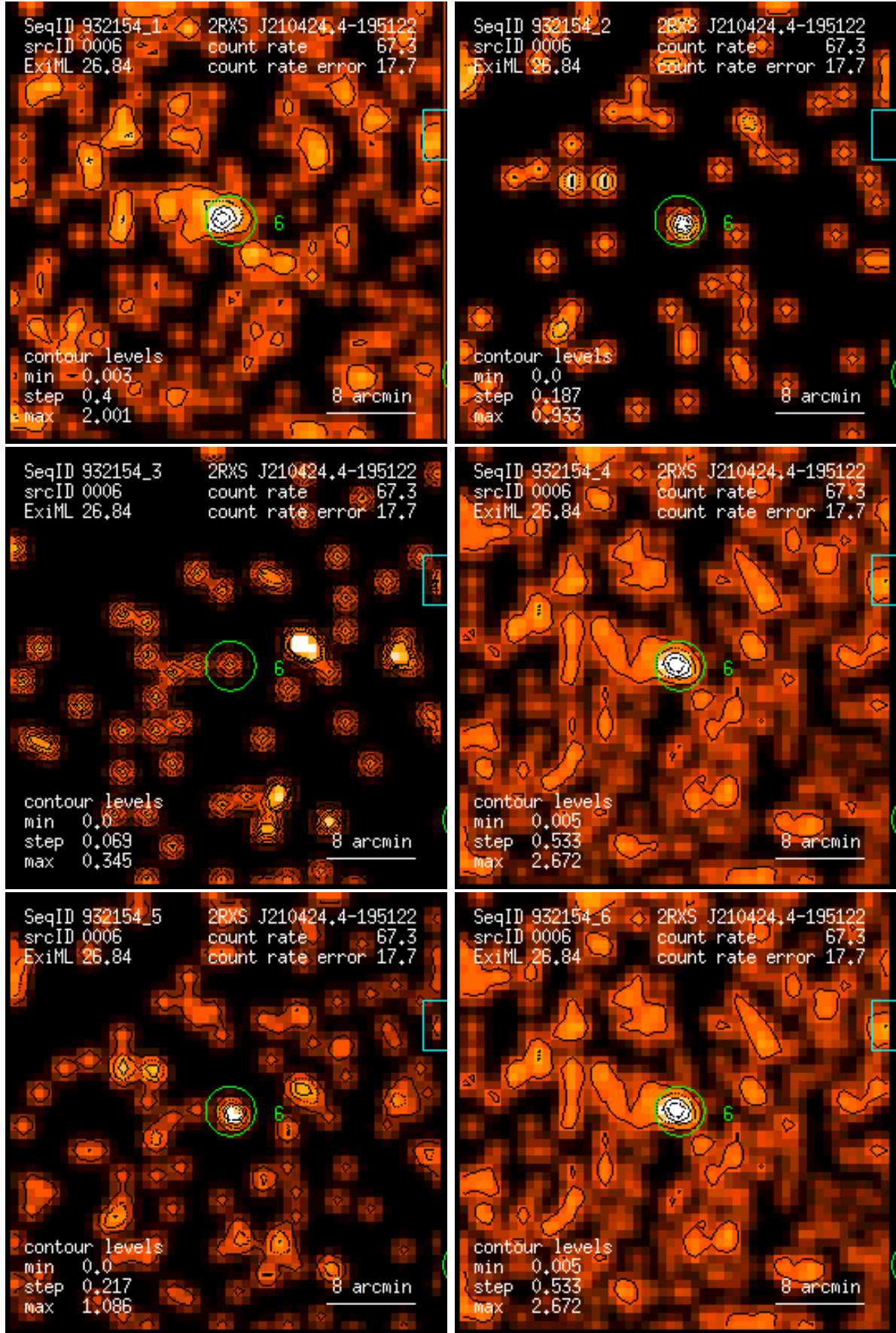
Figure 6: RASS 932154: detection 0006: band rate images, Gaussian filter: (1) PSPC channels 11 – 41, (2) 52 – 90, (3) 91 – 201, (4) 11 – 235, (5) 52 – 201, (6) 11 – 201. Broad band rates in counts/ks. Band rate contour levels in counts/ks/arcmin 2 .
