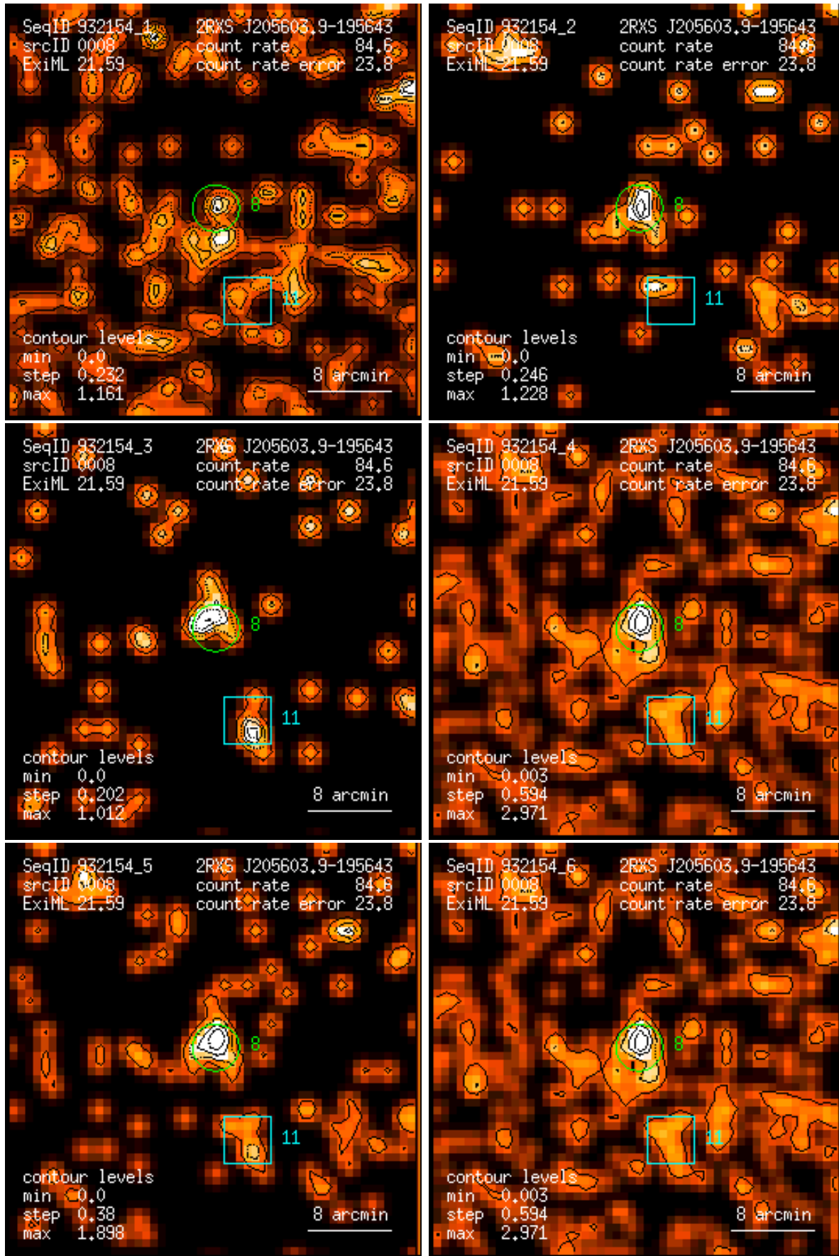
Figure 8: RASS 932154: detection 0008: band rate images, Gaussian filter: (1) PSPC channels 11 – 41, (2) 52 – 90, (3) 91 – 201, (4) 11 – 235, (5) 52 – 201, (6) 11 – 201. Broad band rates in counts/ks. Band rate contour levels in counts/ks/arcmin 2 .
