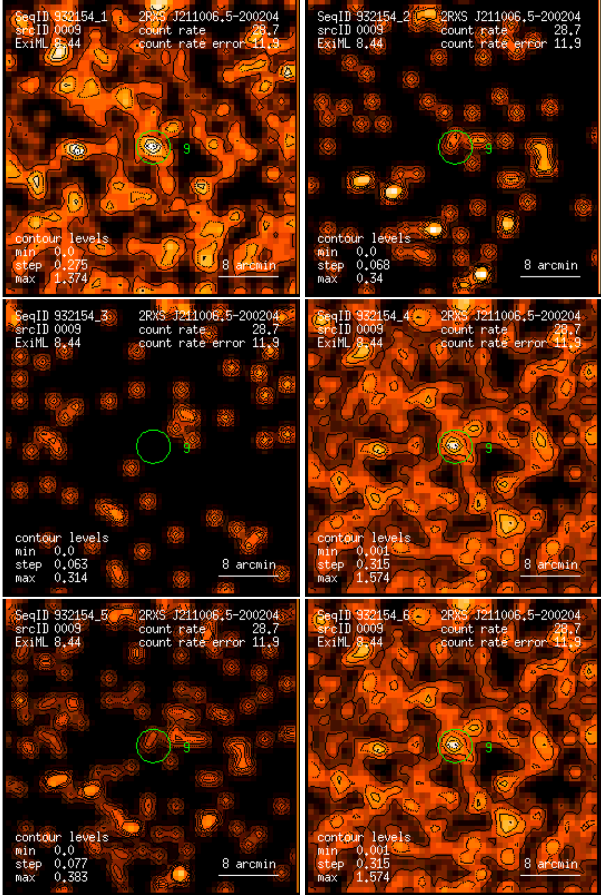
Figure 9: RASS 932154: detection 0009: band rate images, Gaussian filter: (1) PSPC channels 11 – 41, (2) 52 – 90, (3) 91 – 201, (4) 11 – 235, (5) 52 – 201, (6) 11 – 201. Broad band rates in counts/ks. Band rate contour levels in counts/ks/arcmin 2 .
