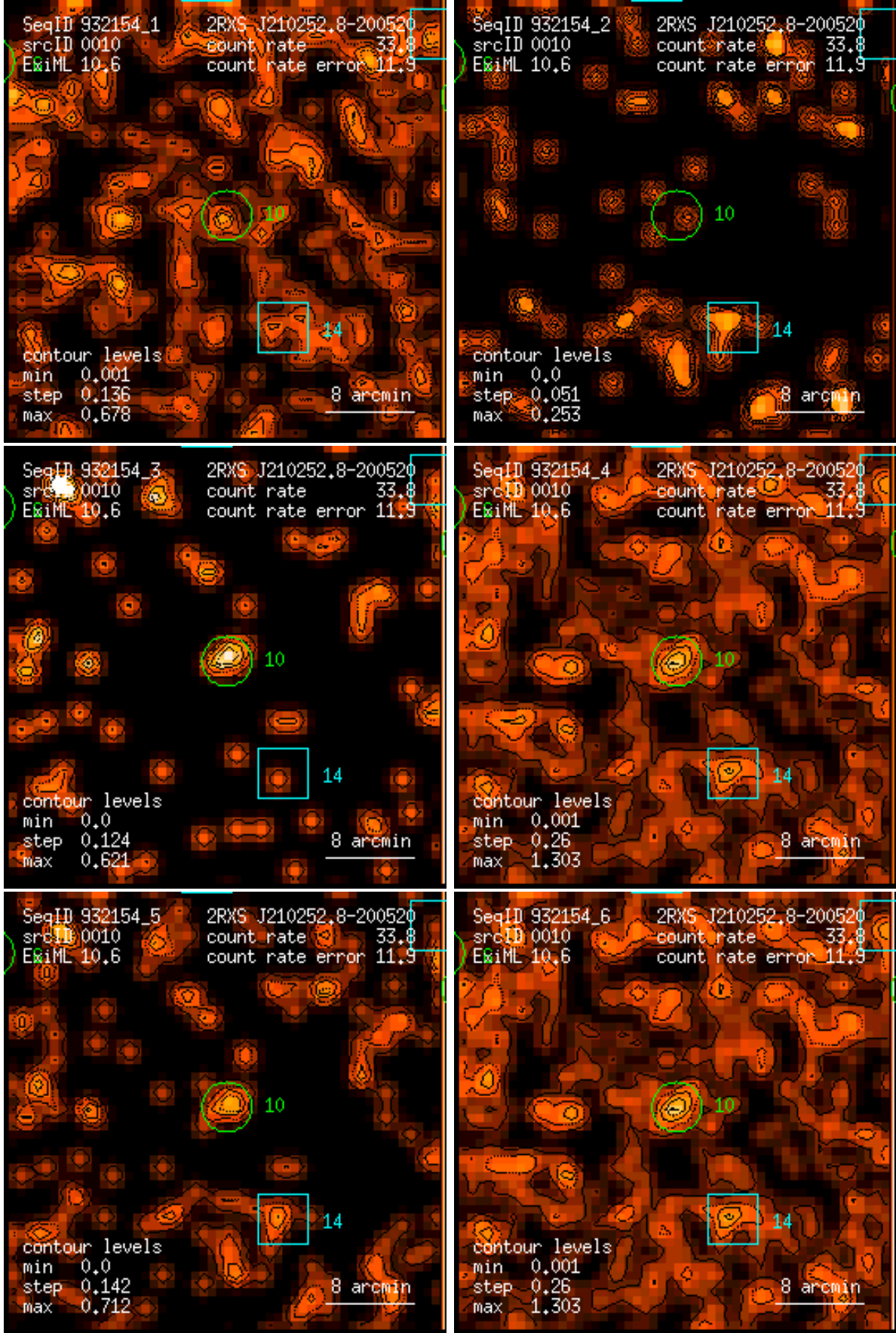
Figure 10: RASS 932154: detection 0010: band rate images, Gaussian filter: (1) PSPC channels 11 – 41, (2) 52 – 90, (3) 91 – 201, (4) 11 – 235, (5) 52 – 201, (6) 11 – 201. Broad band rates in counts/ks. Band rate contour levels in counts/ks/arcmin 2 .
