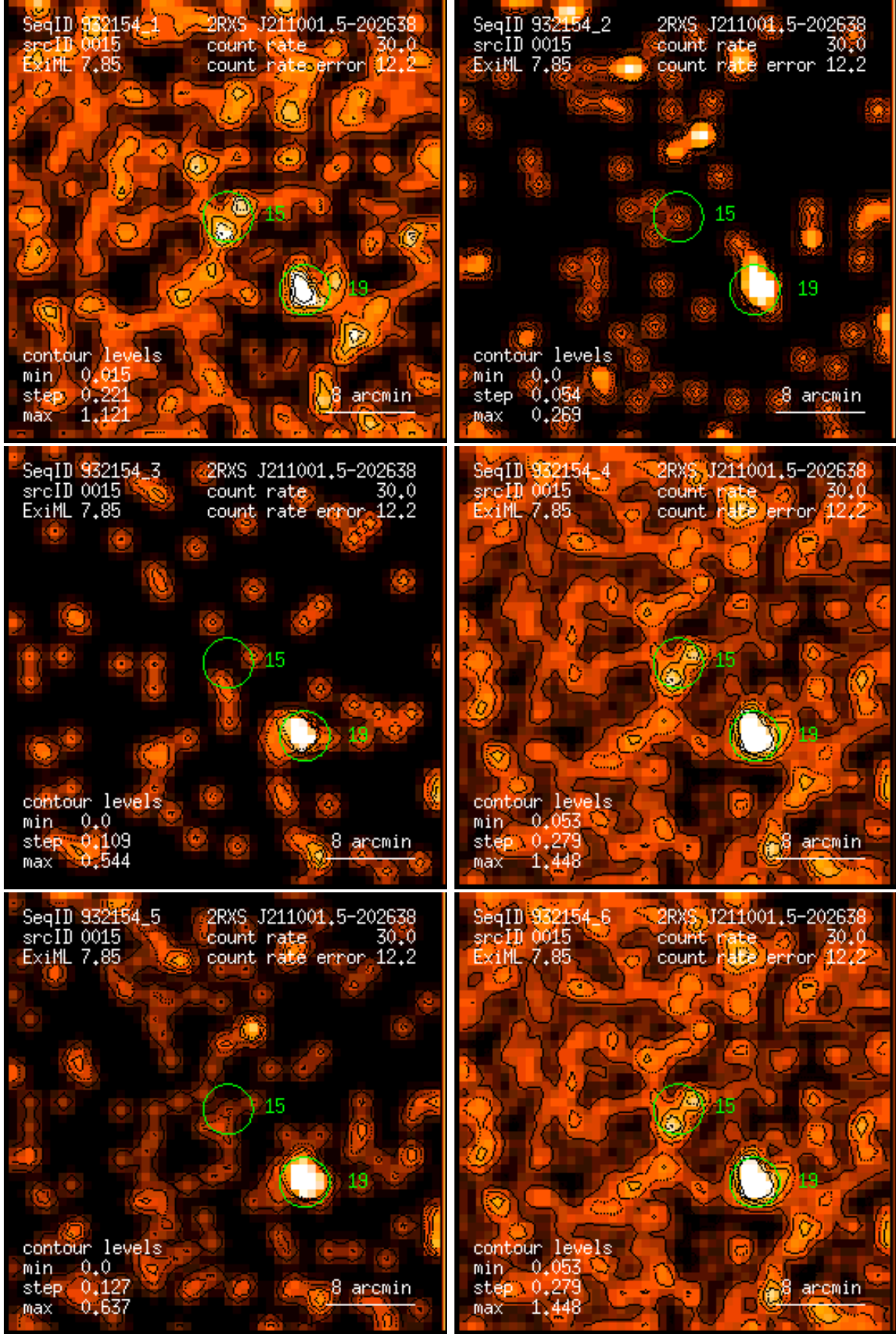
Figure 15: RASS 932154: detection 0015: band rate images, Gaussian filter: (1) PSPC channels 11 – 41, (2) 52 – 90, (3) 91 – 201, (4) 11 – 235, (5) 52 – 201, (6) 11 – 201. Broad band rates in counts/ks. Band rate contour levels in counts/ks/arcmin 2 .
