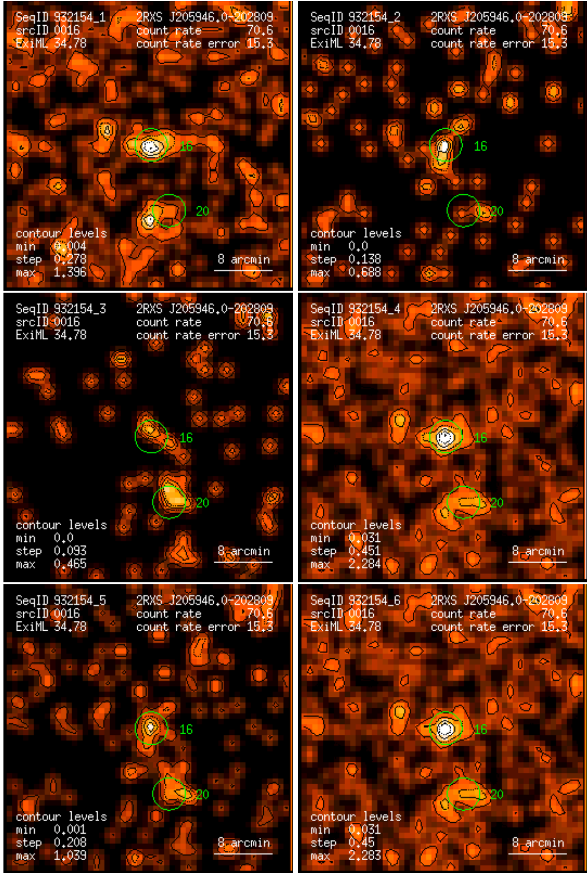
Figure 16: RASS 932154: detection 0016: band rate images, Gaussian filter: (1) PSPC channels 11 – 41, (2) 52 – 90, (3) 91 – 201, (4) 11 – 235, (5) 52 – 201, (6) 11 – 201. Broad band rates in counts/ks. Band rate contour levels in counts/ks/arcmin 2 .
