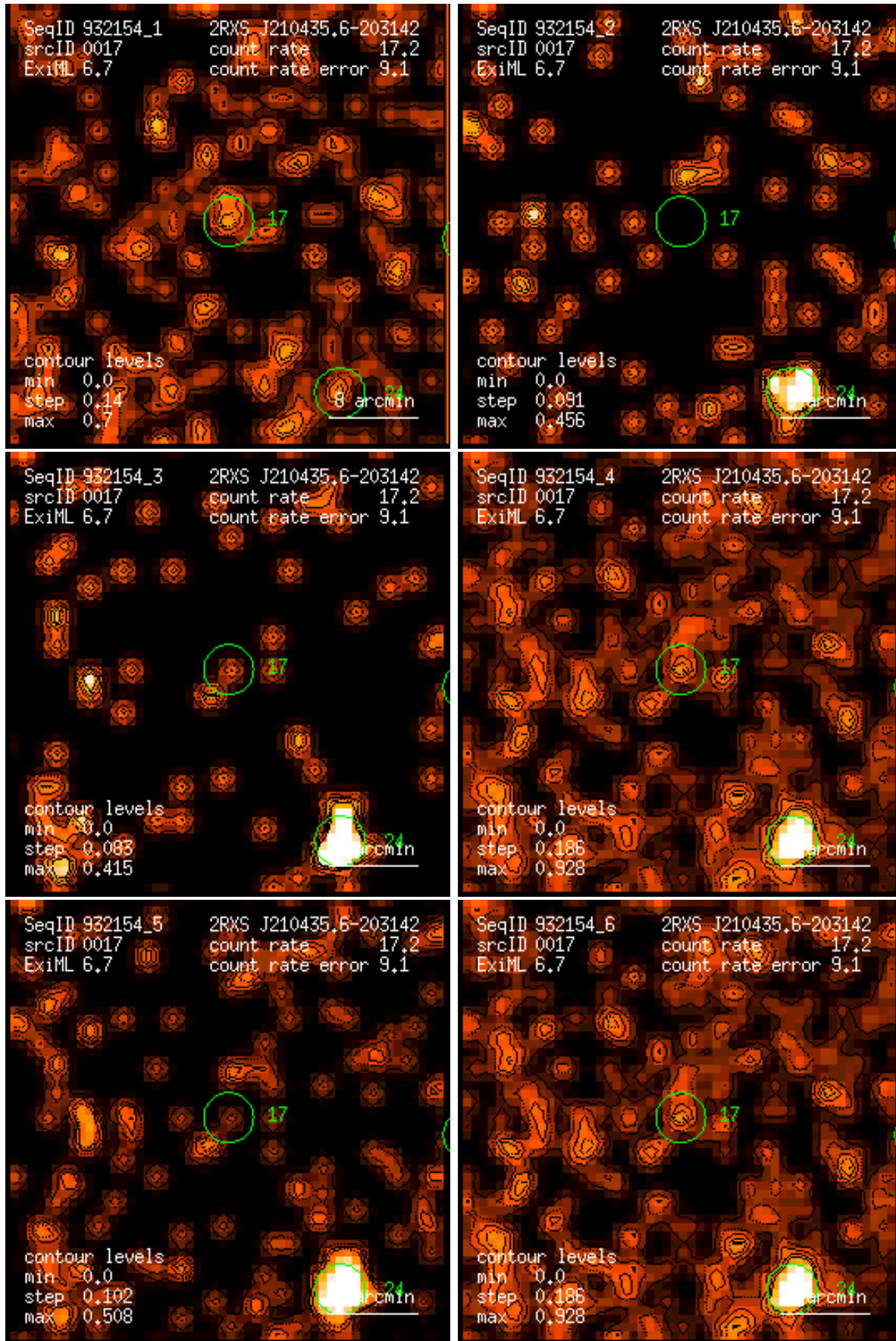
Figure 17: RASS 932154: detection 0017: band rate images, Gaussian filter: (1) PSPC channels 11 – 41, (2) 52 – 90, (3) 91 – 201, (4) 11 – 235, (5) 52 – 201, (6) 11 – 201. Broad band rates in counts/ks. Band rate contour levels in counts/ks/arcmin 2 .
