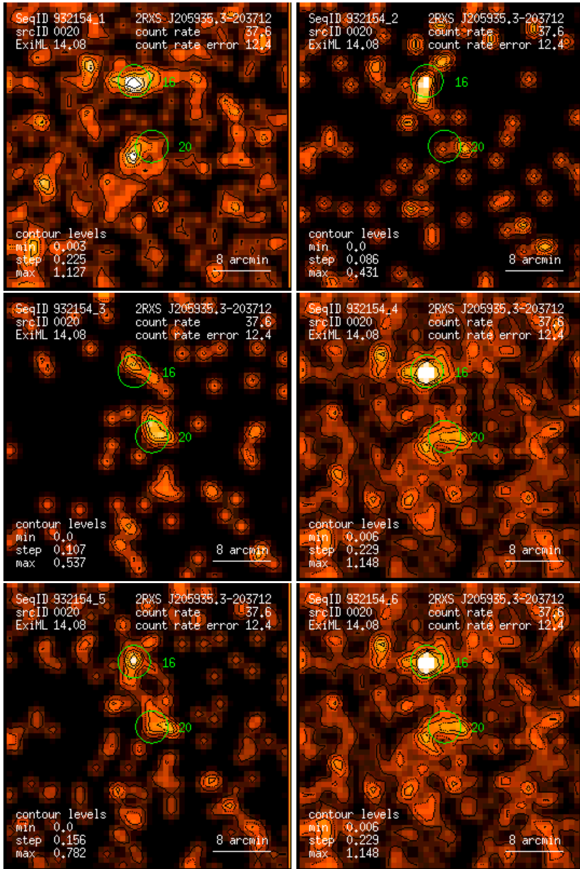
Figure 20: RASS 932154: detection 0020: band rate images, Gaussian filter: (1) PSPC channels 11 – 41, (2) 52 – 90, (3) 91 – 201, (4) 11 – 235, (5) 52 – 201, (6) 11 – 201. Broad band rates in counts/ks. Band rate contour levels in counts/ks/arcmin 2 .
