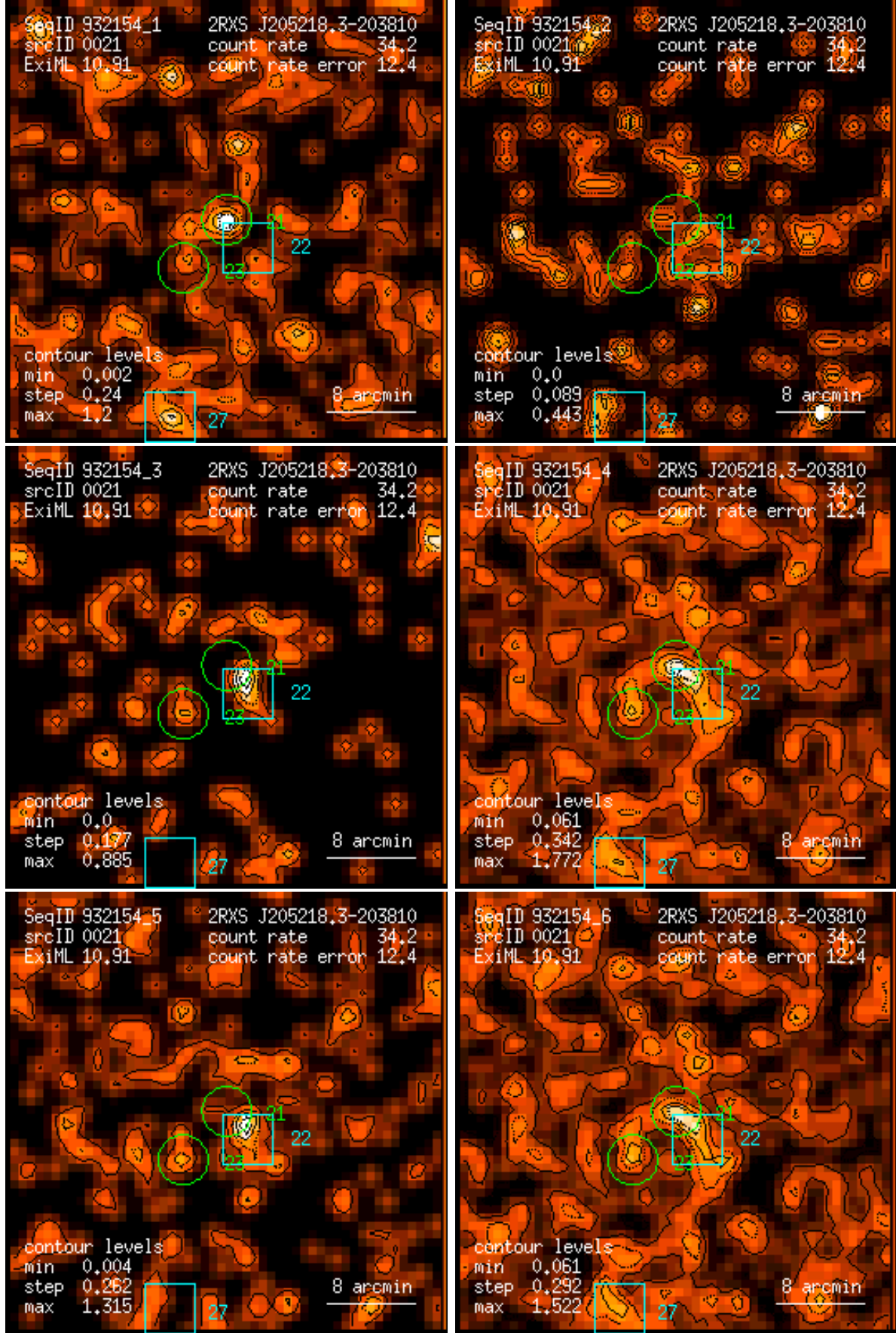
Figure 21: RASS 932154: detection 0021: band rate images, Gaussian filter: (1) PSPC channels 11 – 41, (2) 52 – 90, (3) 91 – 201, (4) 11 – 235, (5) 52 – 201, (6) 11 – 201. Broad band rates in counts/ks. Band rate contour levels in counts/ks/arcmin 2 .
