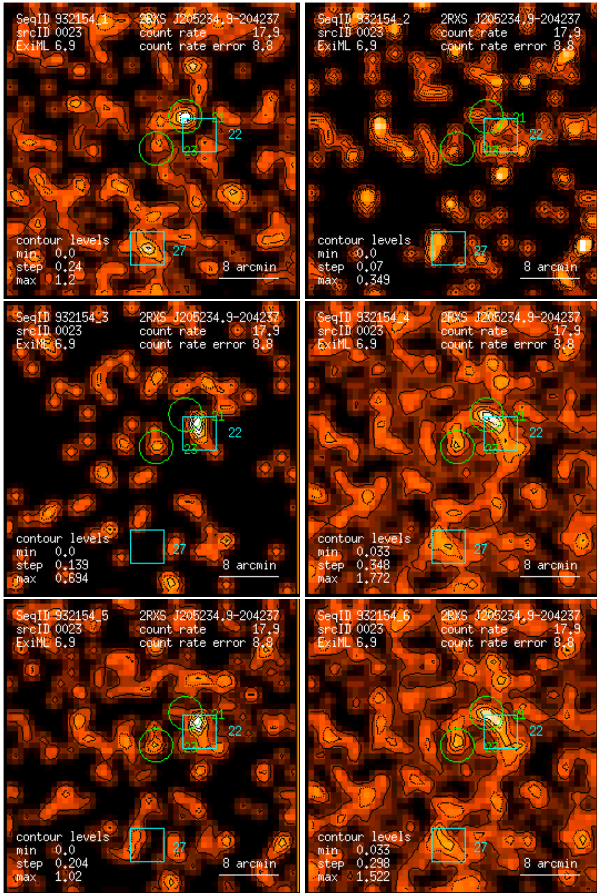
Figure 23: RASS 932154: detection 0023: band rate images, Gaussian filter: (1) PSPC channels 11 – 41, (2) 52 – 90, (3) 91 – 201, (4) 11 – 235, (5) 52 – 201, (6) 11 – 201. Broad band rates in counts/ks. Band rate contour levels in counts/ks/arcmin 2 .
