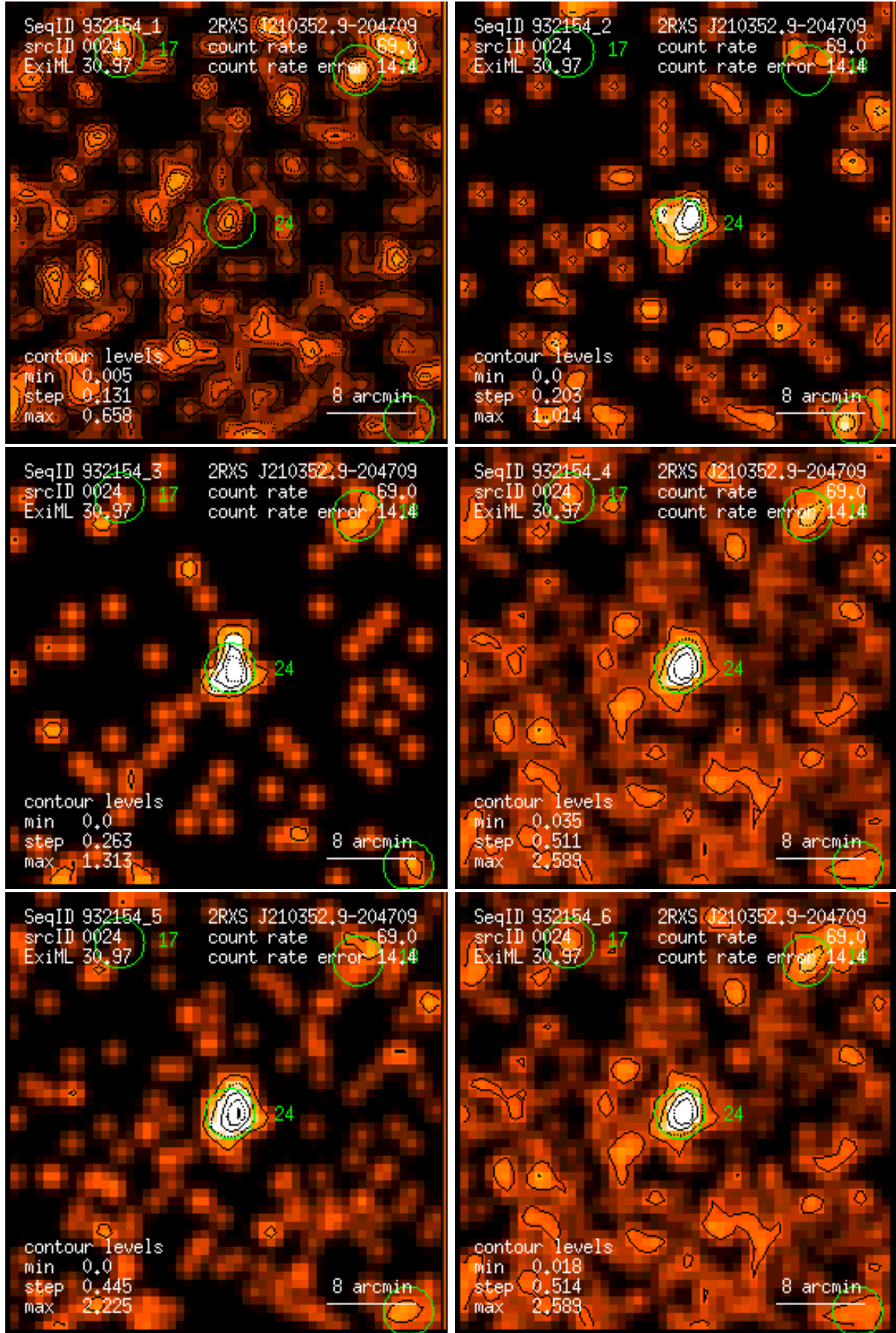
Figure 24: RASS 932154: detection 0024: band rate images, Gaussian filter: (1) PSPC channels 11 – 41, (2) 52 – 90, (3) 91 – 201, (4) 11 – 235, (5) 52 – 201, (6) 11 – 201. Broad band rates in counts/ks. Band rate contour levels in counts/ks/arcmin 2 .
