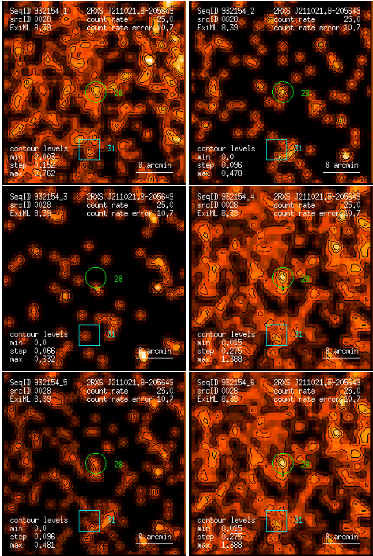
Figure 28: RASS 932154: detection 0028: band rate images, Gaussian filter: (1) PSPC channels 11 – 41, (2) 52 – 90, (3) 91 – 201, (4) 11 – 235, (5) 52 – 201, (6) 11 – 201. Broad band rates in counts/ks. Band rate contour levels in counts/ks/arcmin 2 .
