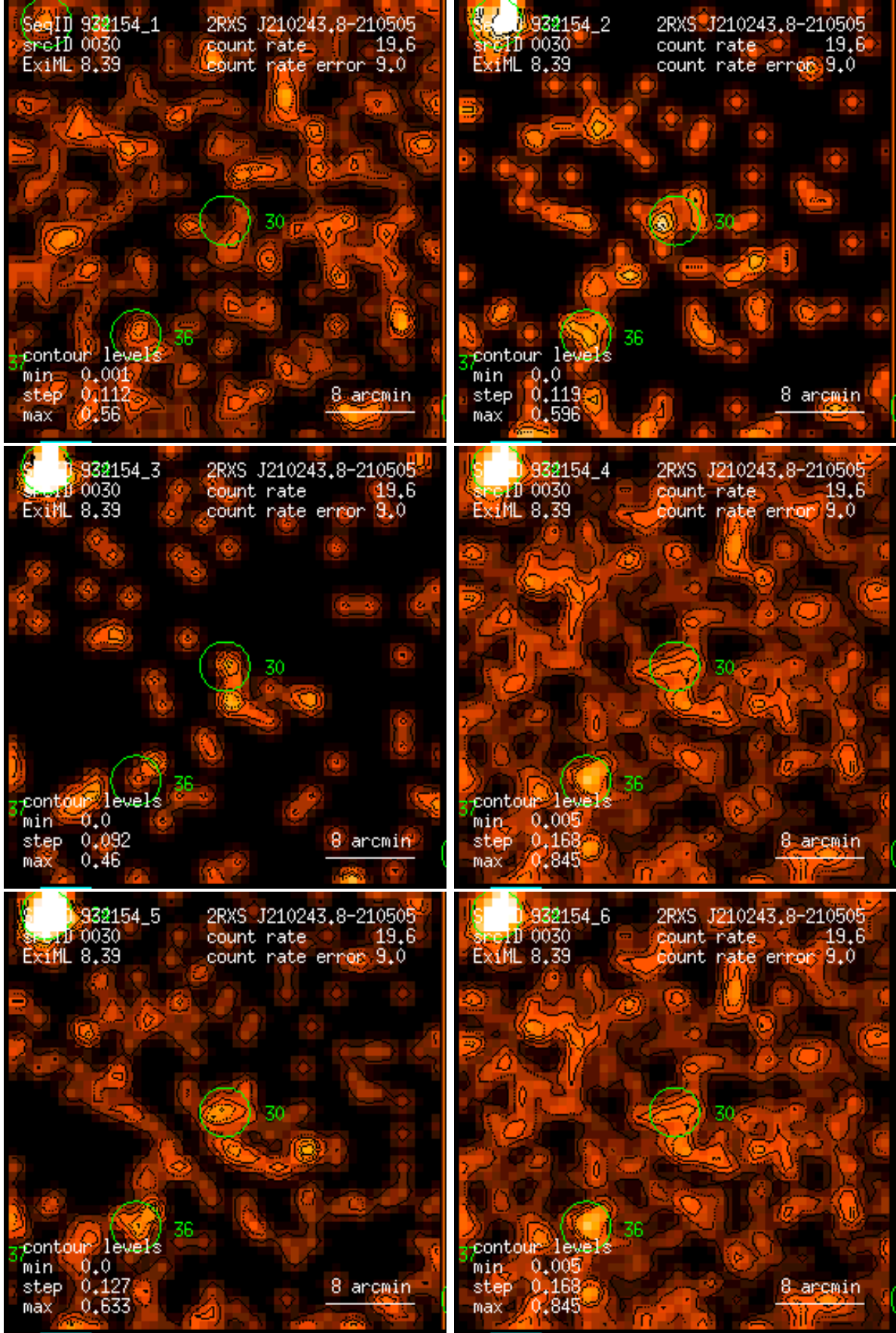
Figure 30: RASS 932154: detection 0030: band rate images, Gaussian filter: (1) PSPC channels 11 – 41, (2) 52 – 90, (3) 91 – 201, (4) 11 – 235, (5) 52 – 201, (6) 11 – 201. Broad band rates in counts/ks. Band rate contour levels in counts/ks/arcmin 2 .
