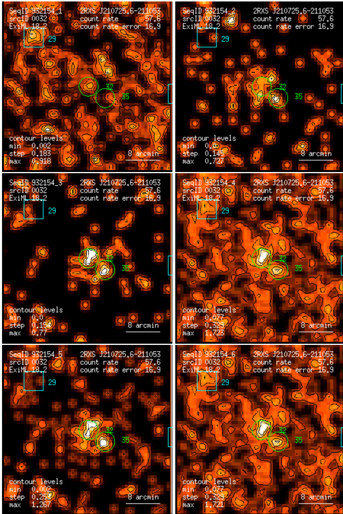
Figure 32: RASS 932154: detection 0032: band rate images, Gaussian filter: (1) PSPC channels 11 – 41, (2) 52 – 90, (3) 91 – 201, (4) 11 – 235, (5) 52 – 201, (6) 11 – 201. Broad band rates in counts/ks. Band rate contour levels in counts/ks/arcmin 2 .
