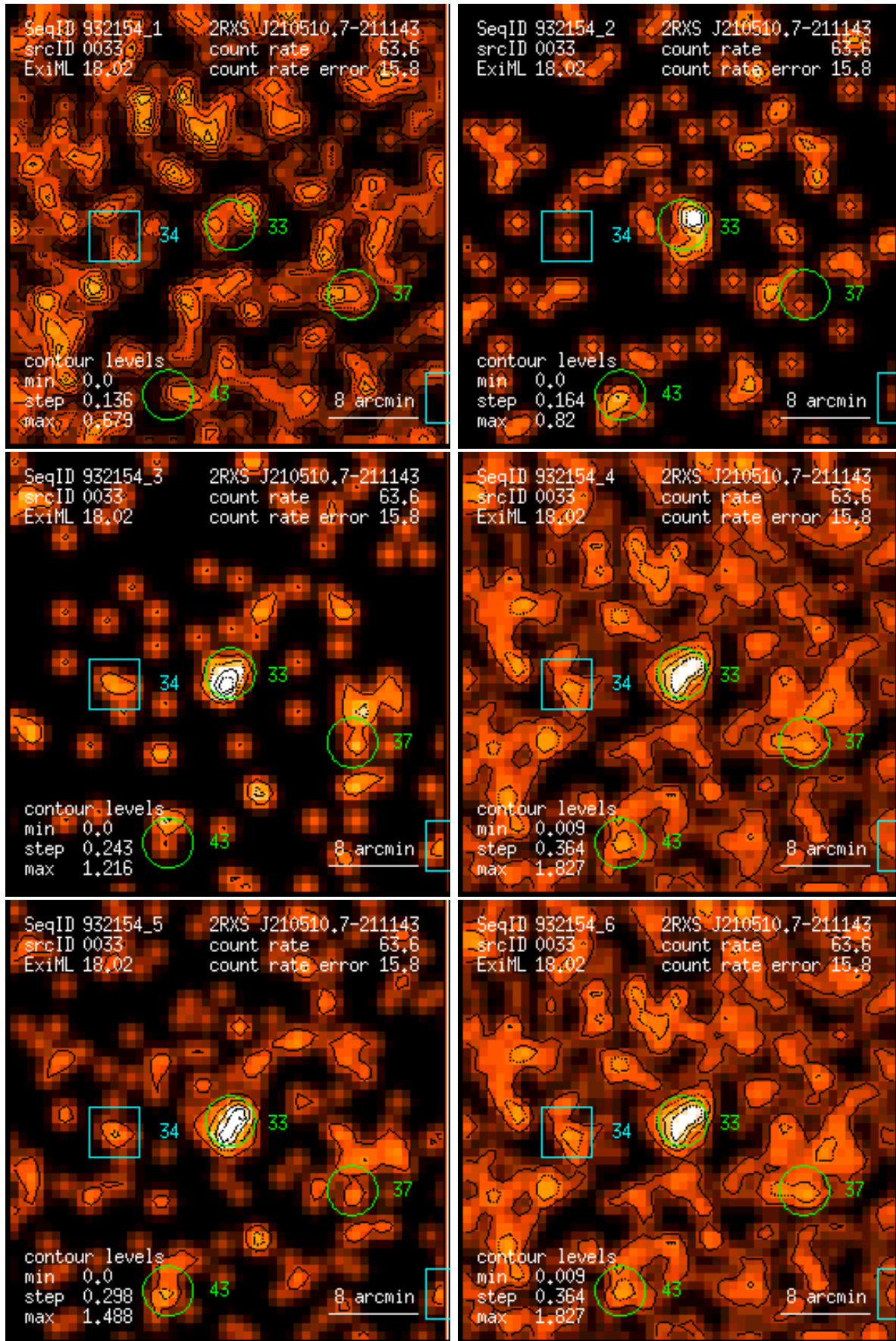
Figure 33: RASS 932154: detection 0033: band rate images, Gaussian filter: (1) PSPC channels 11 – 41, (2) 52 – 90, (3) 91 – 201, (4) 11 – 235, (5) 52 – 201, (6) 11 – 201. Broad band rates in counts/ks. Band rate contour levels in counts/ks/arcmin 2 .
