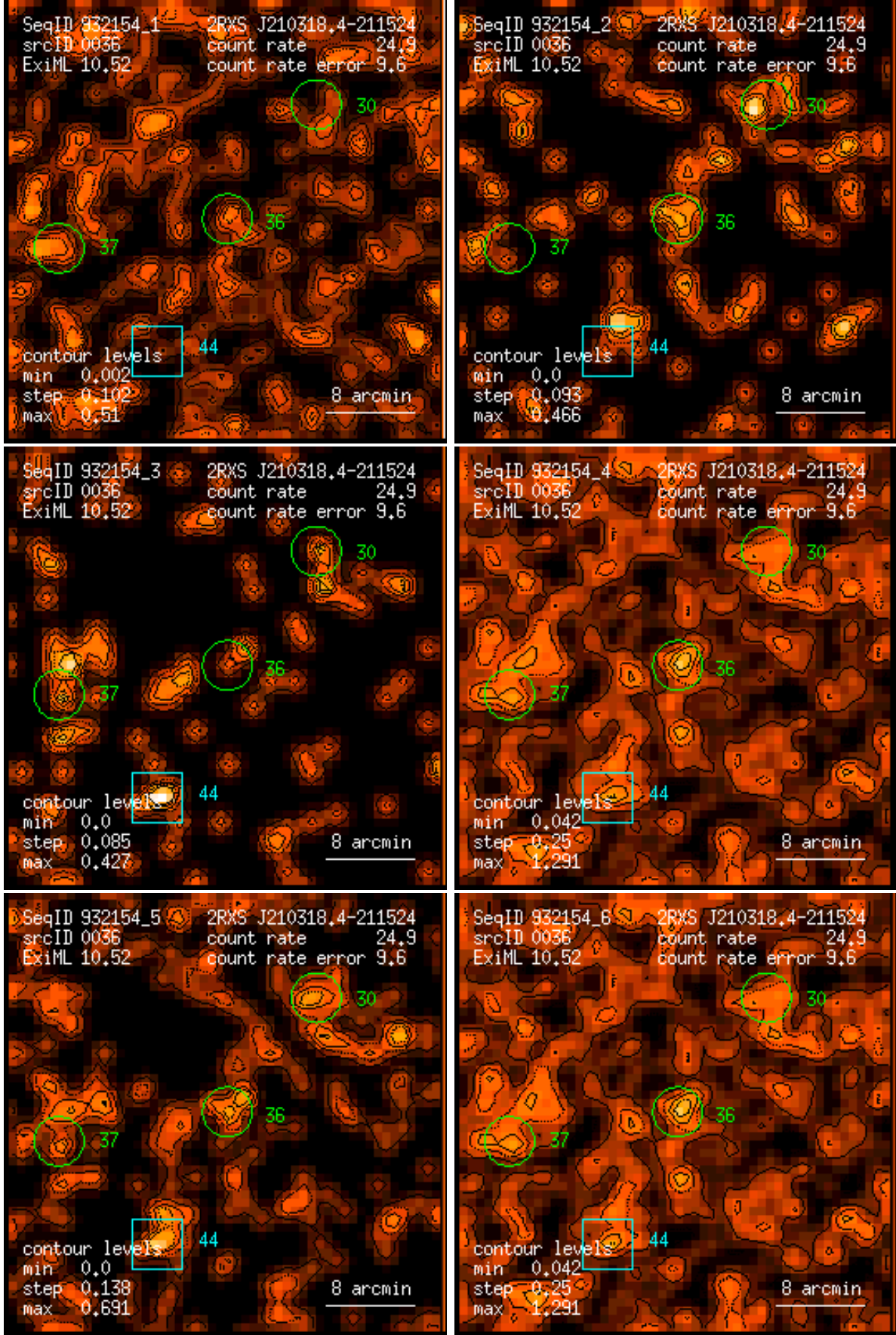
Figure 36: RASS 932154: detection 0036: band rate images, Gaussian filter: (1) PSPC channels 11 – 41, (2) 52 – 90, (3) 91 – 201, (4) 11 – 235, (5) 52 – 201, (6) 11 – 201. Broad band rates in counts/ks. Band rate contour levels in counts/ks/arcmin 2 .
