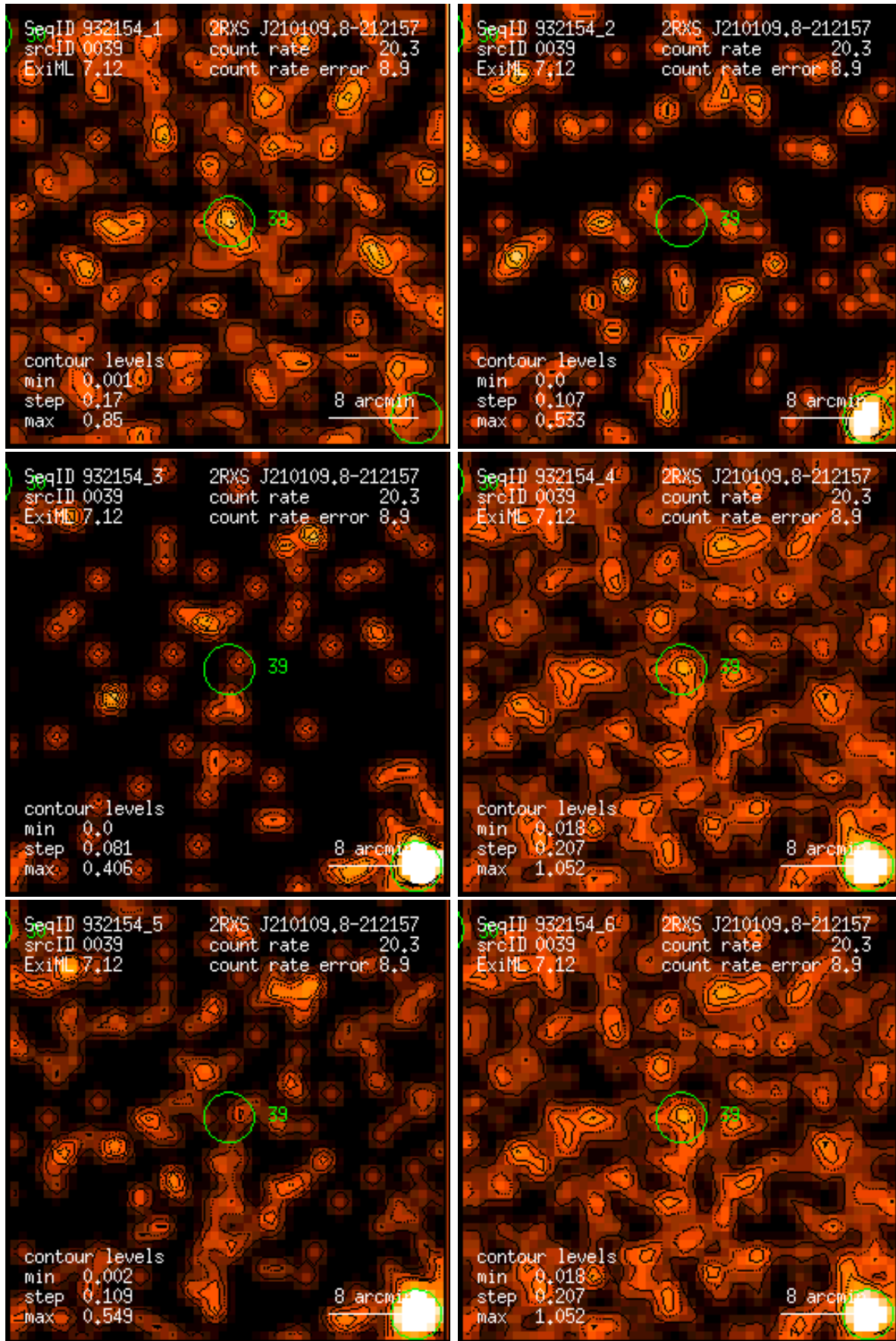
Figure 39: RASS 932154: detection 0039: band rate images, Gaussian filter: (1) PSPC channels 11 – 41, (2) 52 – 90, (3) 91 – 201, (4) 11 – 235, (5) 52 – 201, (6) 11 – 201. Broad band rates in counts/ks. Band rate contour levels in counts/ks/arcmin 2 .
