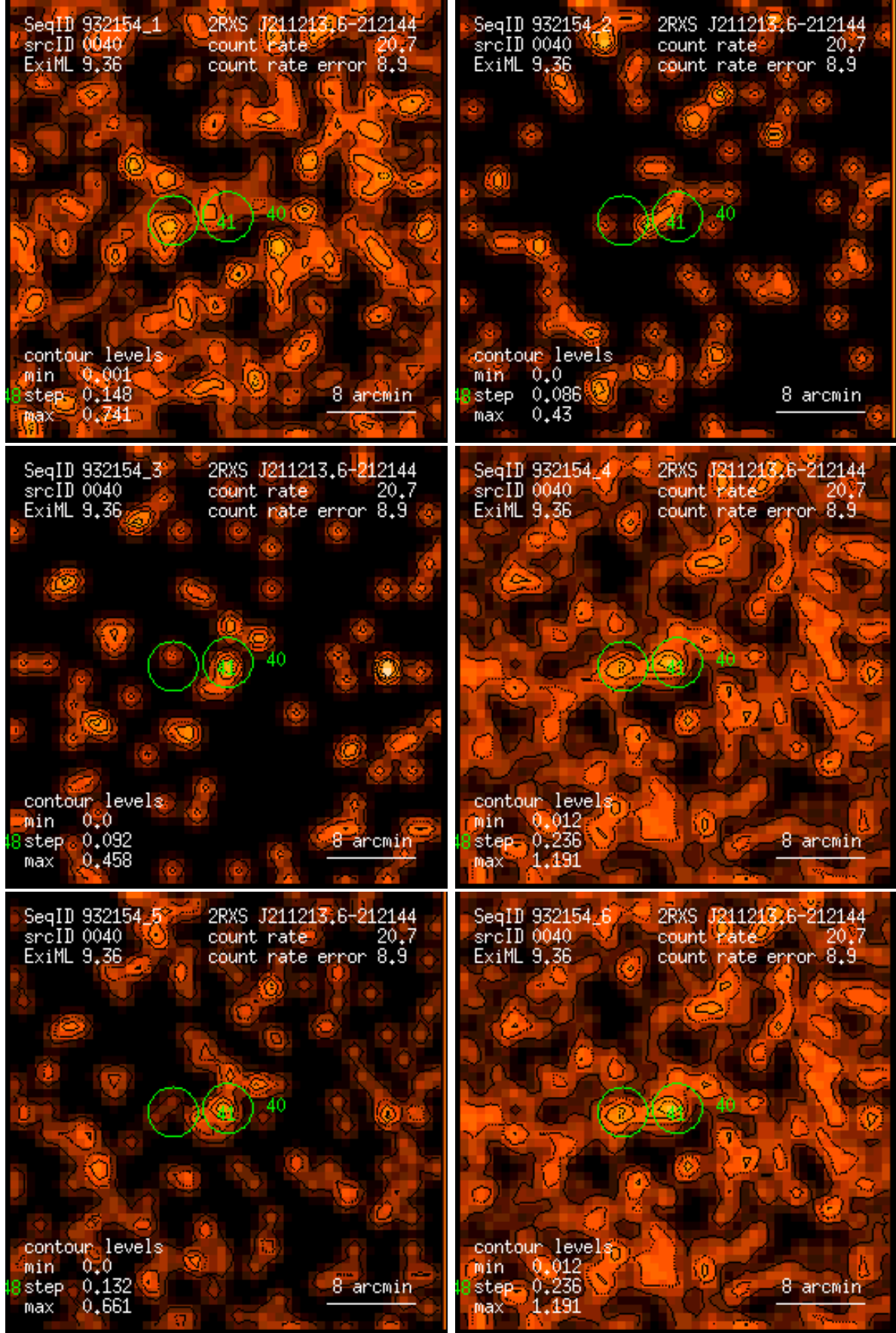
Figure 40: RASS 932154: detection 0040: band rate images, Gaussian filter: (1) PSPC channels 11 – 41, (2) 52 – 90, (3) 91 – 201, (4) 11 – 235, (5) 52 – 201, (6) 11 – 201. Broad band rates in counts/ks. Band rate contour levels in counts/ks/arcmin 2 .
