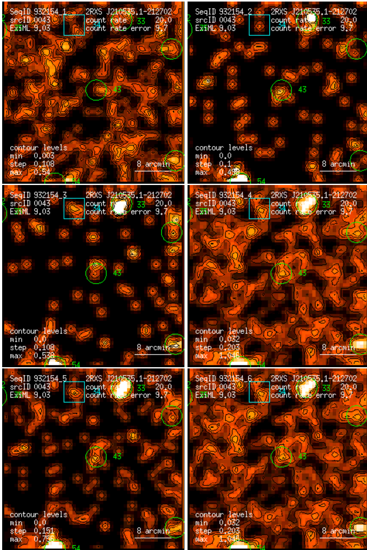
Figure 43: RASS 932154: detection 0043: band rate images, Gaussian filter: (1) PSPC channels 11 – 41, (2) 52 – 90, (3) 91 – 201, (4) 11 – 235, (5) 52 – 201, (6) 11 – 201. Broad band rates in counts/ks. Band rate contour levels in counts/ks/arcmin 2 .
