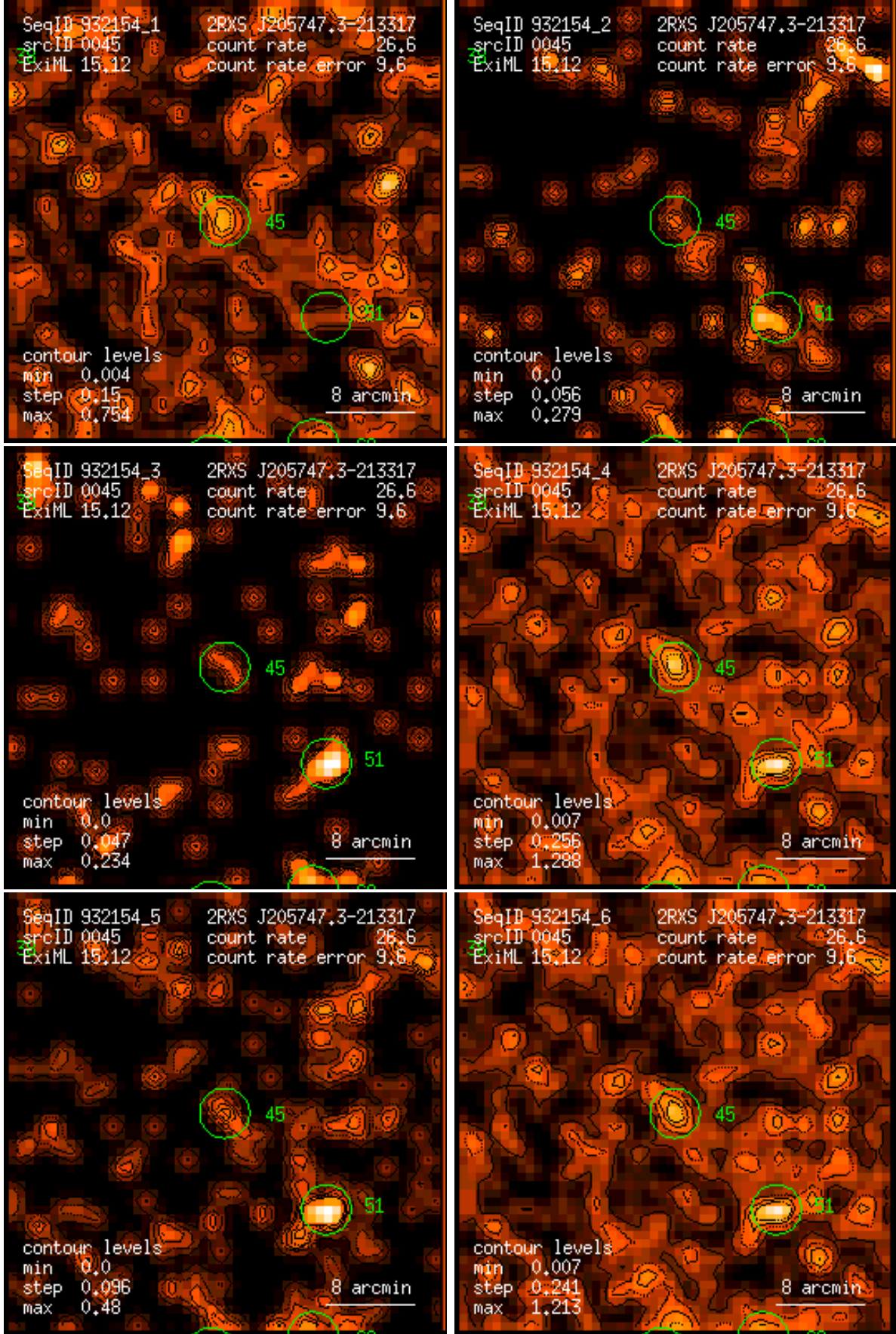
Figure 45: RASS 932154: detection 0045: band rate images, Gaussian filter: (1) PSPC channels 11 – 41, (2) 52 – 90, (3) 91 – 201, (4) 11 – 235, (5) 52 – 201, (6) 11 – 201. Broad band rates in counts/ks. Band rate contour levels in counts/ks/arcmin 2 .
