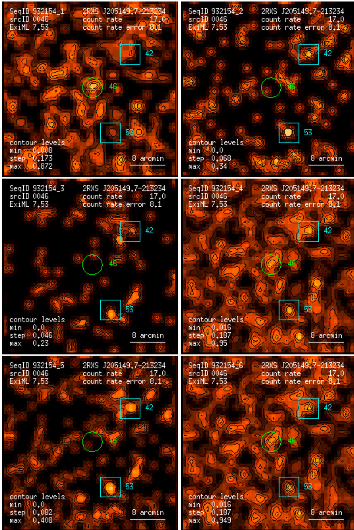
Figure 46: RASS 932154: detection 0046: band rate images, Gaussian filter: (1) PSPC channels 11 – 41, (2) 52 – 90, (3) 91 – 201, (4) 11 – 235, (5) 52 – 201, (6) 11 – 201. Broad band rates in counts/ks. Band rate contour levels in counts/ks/arcmin 2 .
