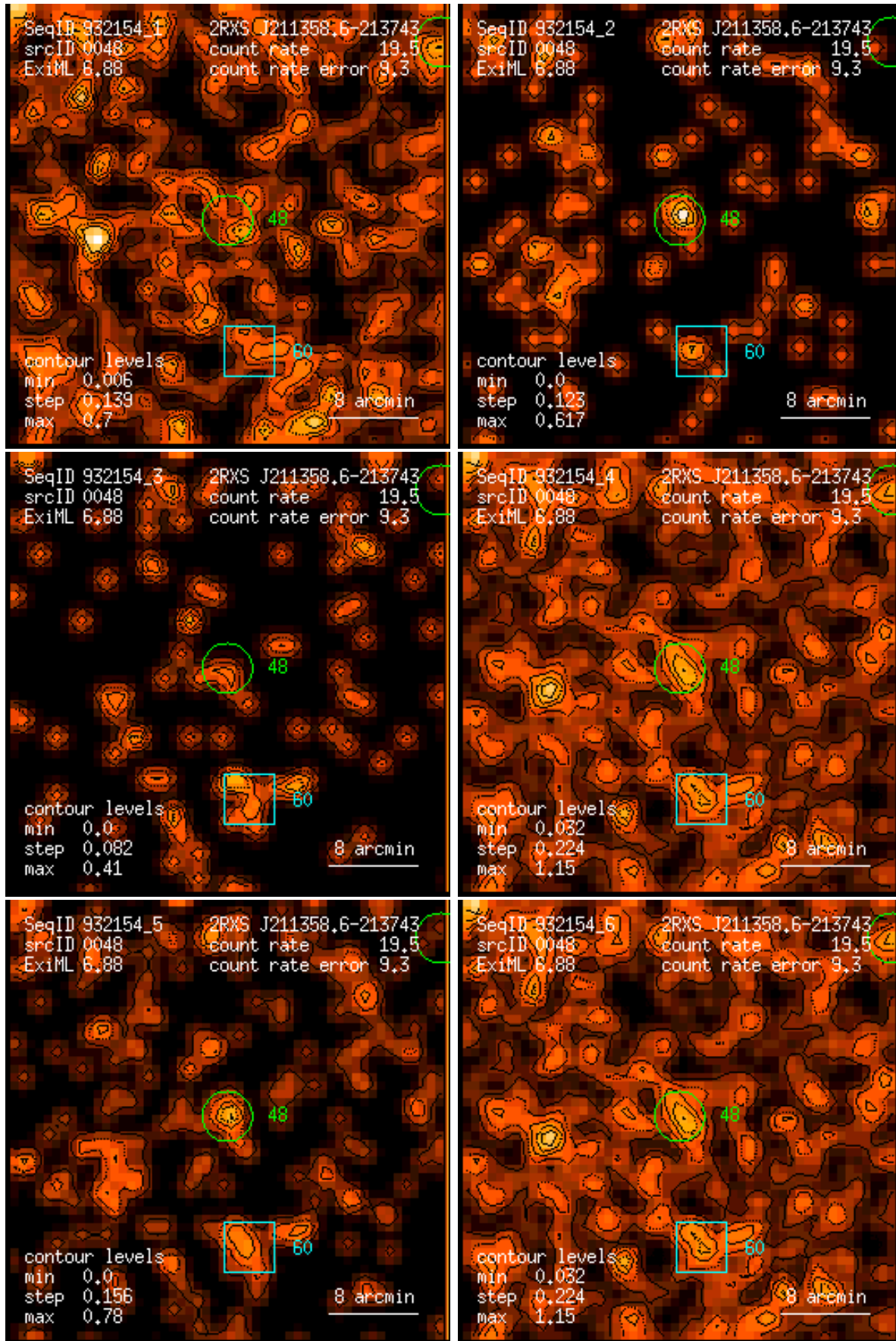
Figure 48: RASS 932154: detection 0048: band rate images, Gaussian filter: (1) PSPC channels 11 – 41, (2) 52 – 90, (3) 91 – 201, (4) 11 – 235, (5) 52 – 201, (6) 11 – 201. Broad band rates in counts/ks. Band rate contour levels in counts/ks/arcmin 2 .
