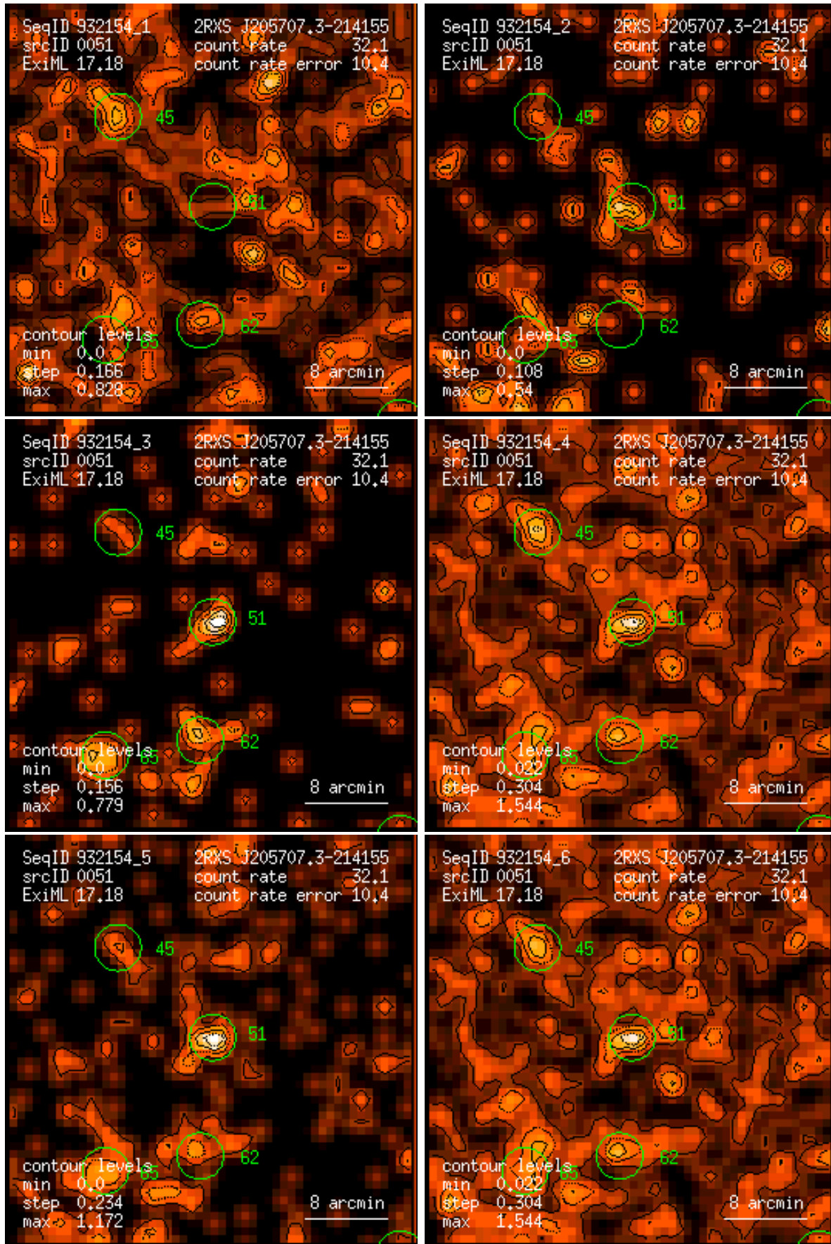
Figure 51: RASS 932154: detection 0051: band rate images, Gaussian filter: (1) PSPC channels 11 – 41, (2) 52 – 90, (3) 91 – 201, (4) 11 – 235, (5) 52 – 201, (6) 11 – 201. Broad band rates in counts/ks. Band rate contour levels in counts/ks/arcmin 2 .
