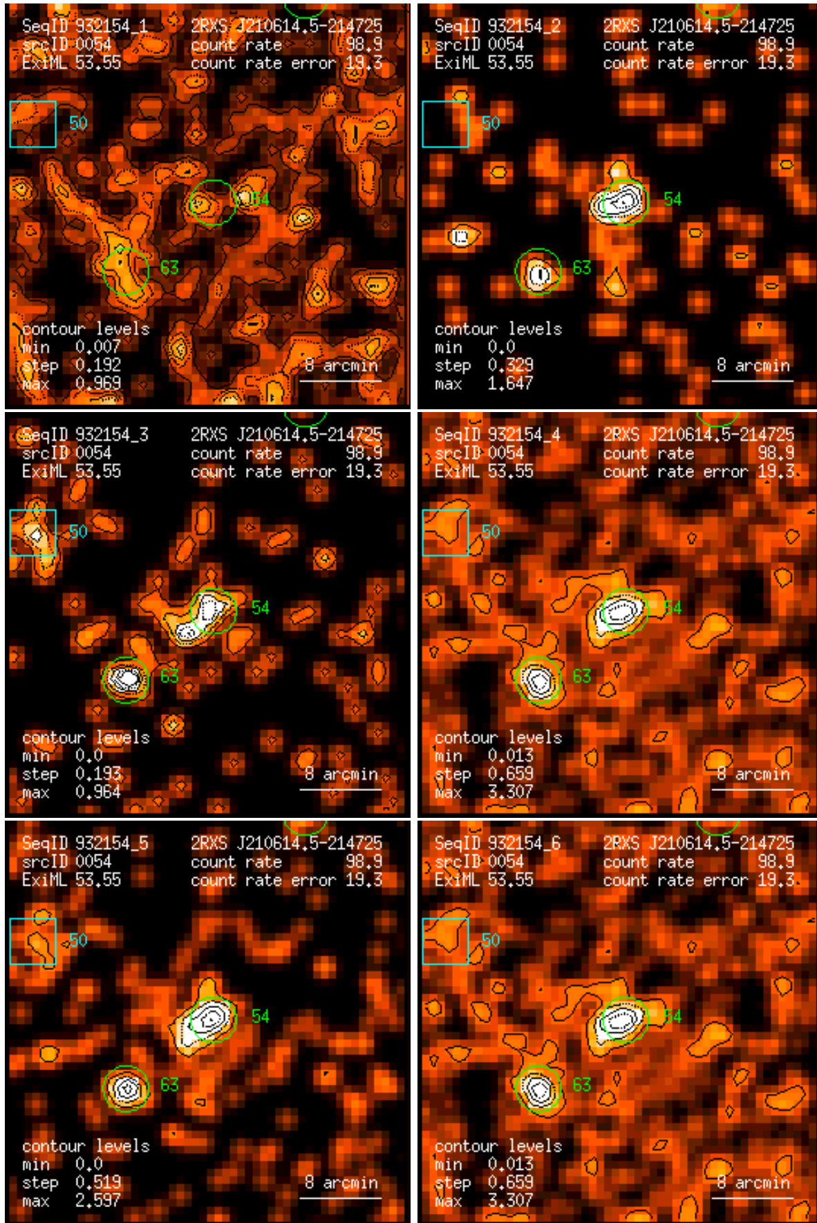
Figure 54: RASS 932154: detection 0054: band rate images, Gaussian filter: (1) PSPC channels 11 – 41, (2) 52 – 90, (3) 91 – 201, (4) 11 – 235, (5) 52 – 201, (6) 11 – 201. Broad band rates in counts/ks. Band rate contour levels in counts/ks/arcmin 2 .
