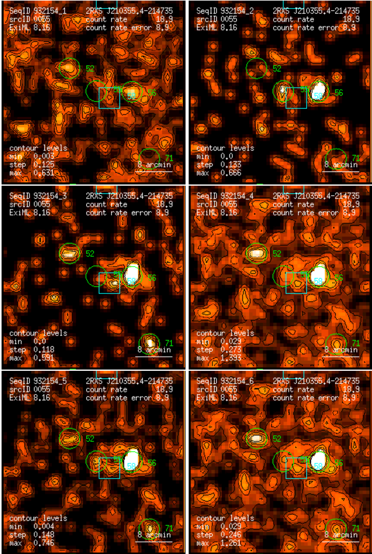
Figure 55: RASS 932154: detection 0055: band rate images, Gaussian filter: (1) PSPC channels 11 – 41, (2) 52 – 90, (3) 91 – 201, (4) 11 – 235, (5) 52 – 201, (6) 11 – 201. Broad band rates in counts/ks. Band rate contour levels in counts/ks/arcmin 2 .
