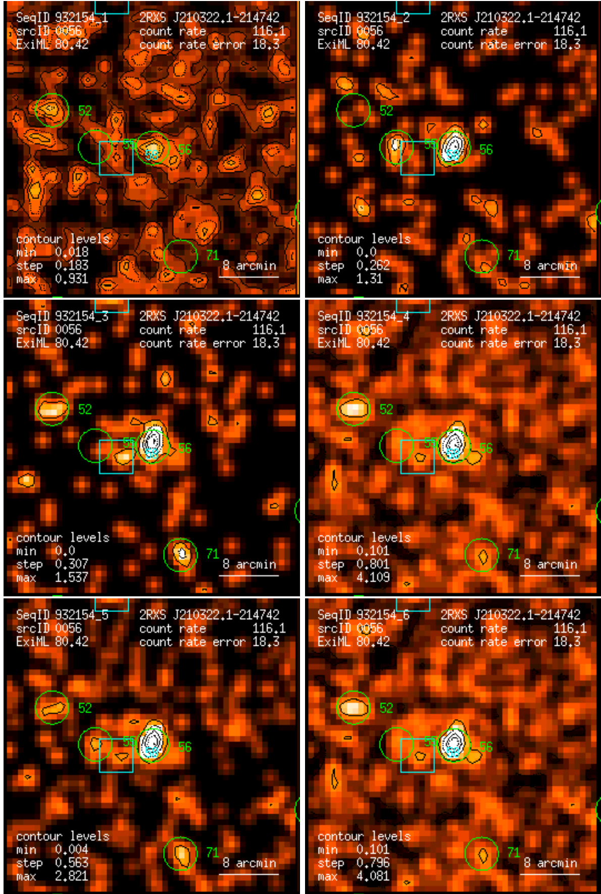
Figure 56: RASS 932154: detection 0056: band rate images, Gaussian filter: (1) PSPC channels 11 – 41, (2) 52 – 90, (3) 91 – 201, (4) 11 – 235, (5) 52 – 201, (6) 11 – 201. Broad band rates in counts/ks. Band rate contour levels in counts/ks/arcmin 2 .
