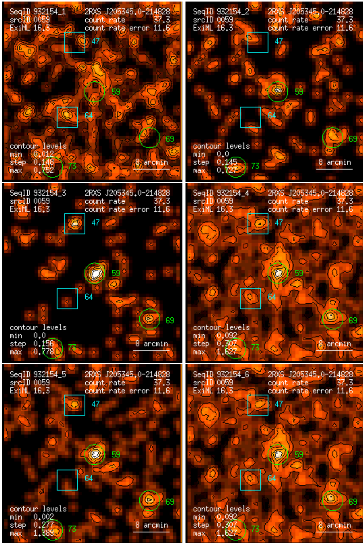
Figure 59: RASS 932154: detection 0059: band rate images, Gaussian filter: (1) PSPC channels 11 – 41, (2) 52 – 90, (3) 91 – 201, (4) 11 – 235, (5) 52 – 201, (6) 11 – 201. Broad band rates in counts/ks. Band rate contour levels in counts/ks/arcmin 2 .
