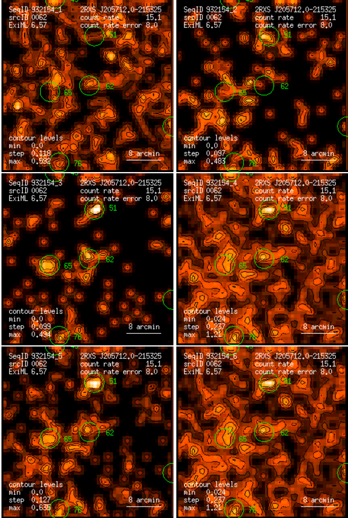
Figure 62: RASS 932154: detection 0062: band rate images, Gaussian filter: (1) PSPC channels 11 – 41, (2) 52 – 90, (3) 91 – 201, (4) 11 – 235, (5) 52 – 201, (6) 11 – 201. Broad band rates in counts/ks. Band rate contour levels in counts/ks/arcmin 2 .
