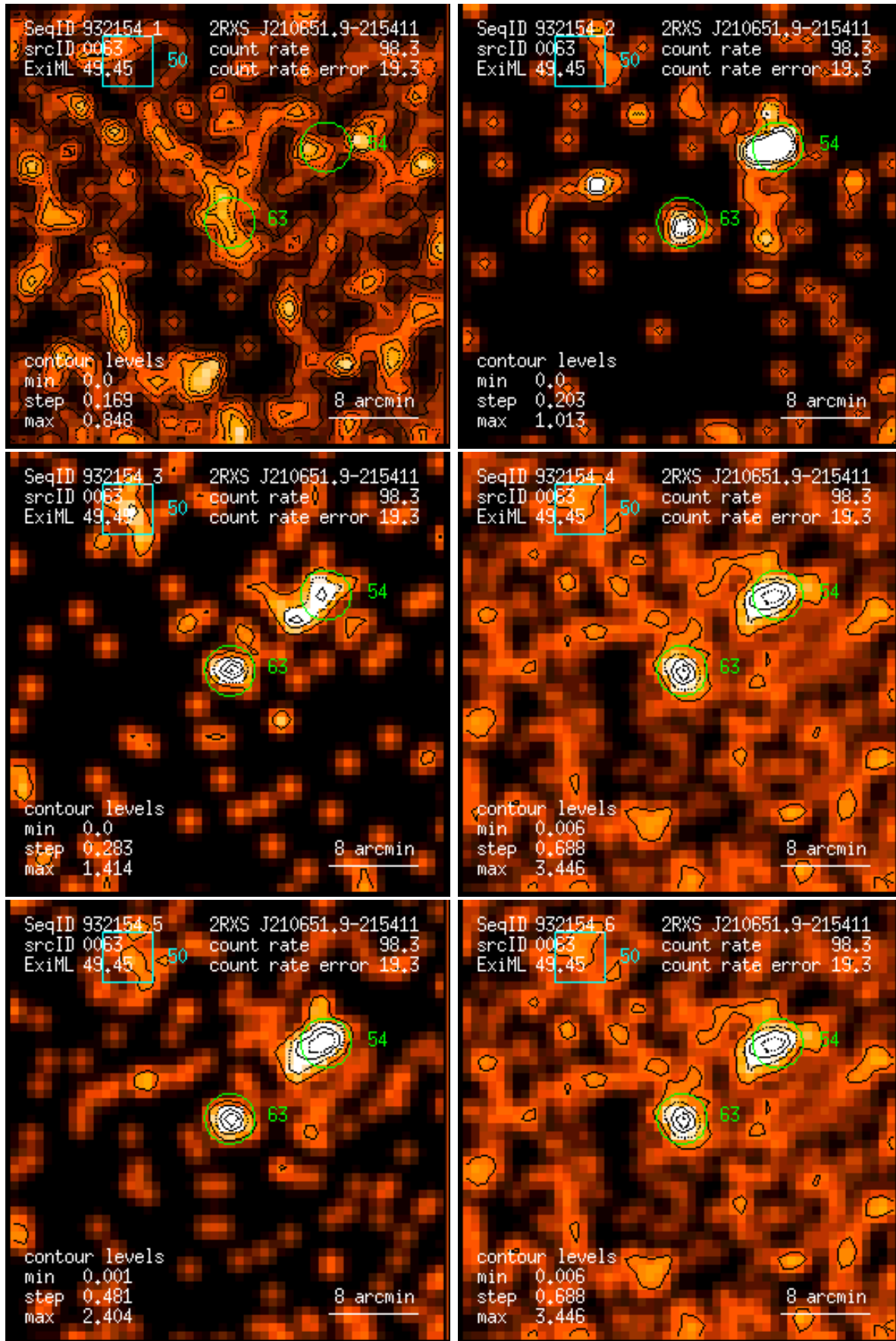
Figure 63: RASS 932154: detection 0063: band rate images, Gaussian filter: (1) PSPC channels 11 – 41, (2) 52 – 90, (3) 91 – 201, (4) 11 – 235, (5) 52 – 201, (6) 11 – 201. Broad band rates in counts/ks. Band rate contour levels in counts/ks/arcmin 2 .
