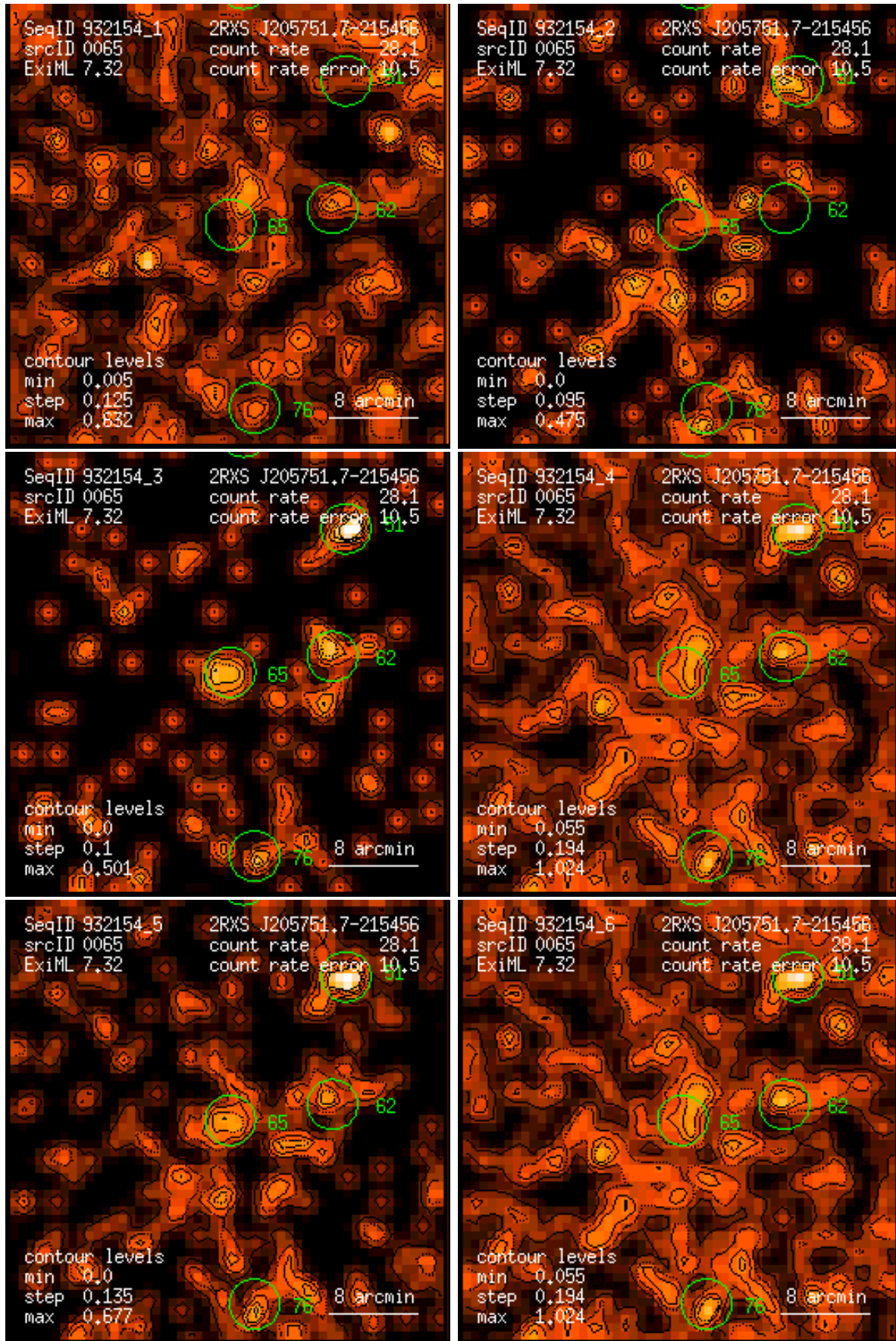
Figure 65: RASS 932154: detection 0065: band rate images, Gaussian filter: (1) PSPC channels 11 – 41, (2) 52 – 90, (3) 91 – 201, (4) 11 – 235, (5) 52 – 201, (6) 11 – 201. Broad band rates in counts/ks. Band rate contour levels in counts/ks/arcmin 2 .
