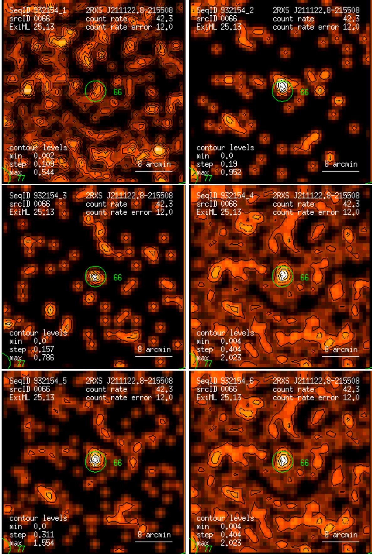
Figure 66: RASS 932154: detection 0066: band rate images, Gaussian filter: (1) PSPC channels 11 – 41, (2) 52 – 90, (3) 91 – 201, (4) 11 – 235, (5) 52 – 201, (6) 11 – 201. Broad band rates in counts/ks. Band rate contour levels in counts/ks/arcmin 2 .
