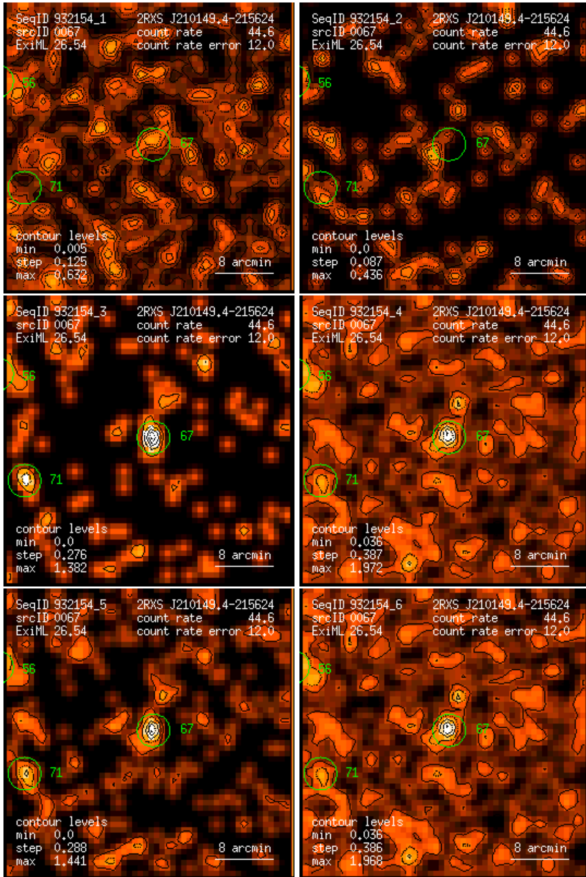
Figure 67: RASS 932154: detection 0067: band rate images, Gaussian filter: (1) PSPC channels 11 – 41, (2) 52 – 90, (3) 91 – 201, (4) 11 – 235, (5) 52 – 201, (6) 11 – 201. Broad band rates in counts/ks. Band rate contour levels in counts/ks/arcmin 2 .
