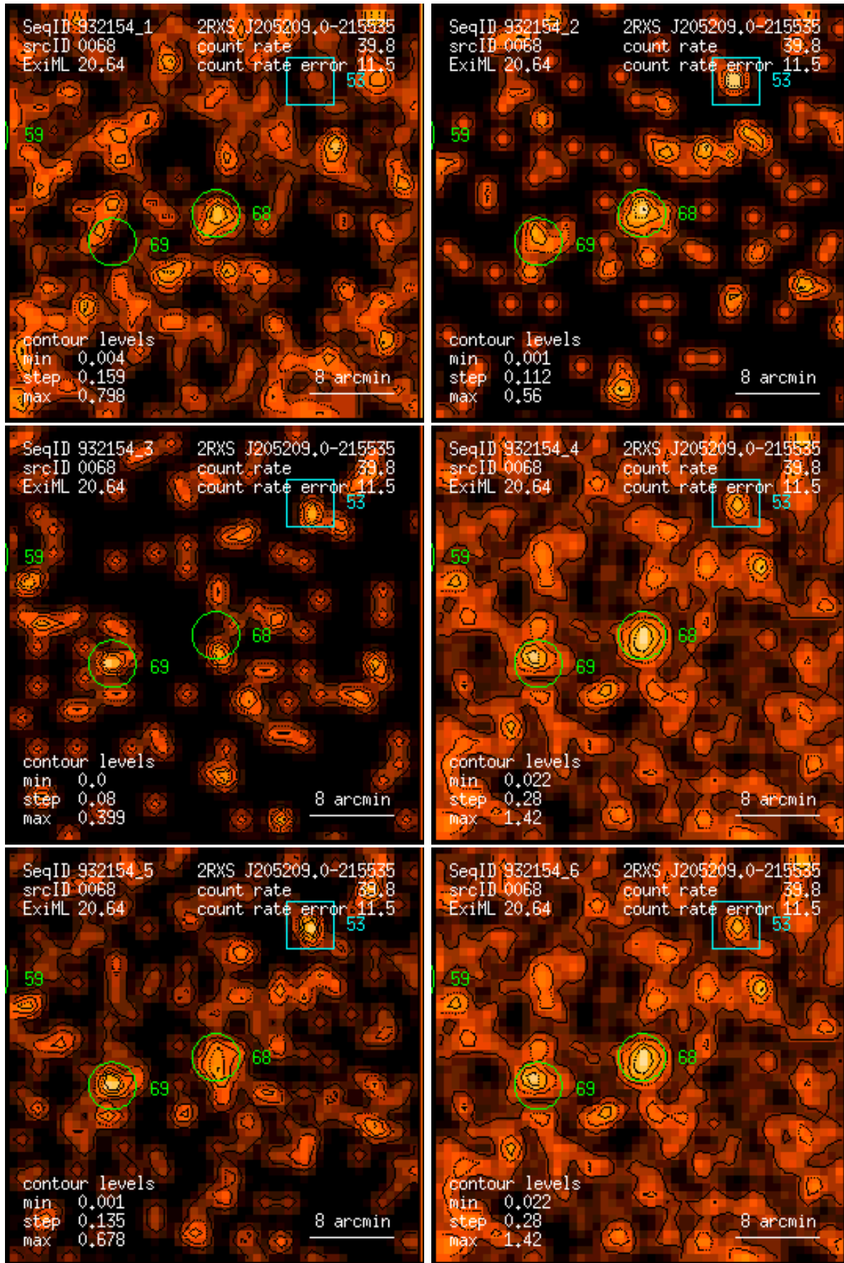
Figure 68: RASS 932154: detection 0068: band rate images, Gaussian filter: (1) PSPC channels 11 – 41, (2) 52 – 90, (3) 91 – 201, (4) 11 – 235, (5) 52 – 201, (6) 11 – 201. Broad band rates in counts/ks. Band rate contour levels in counts/ks/arcmin 2 .
