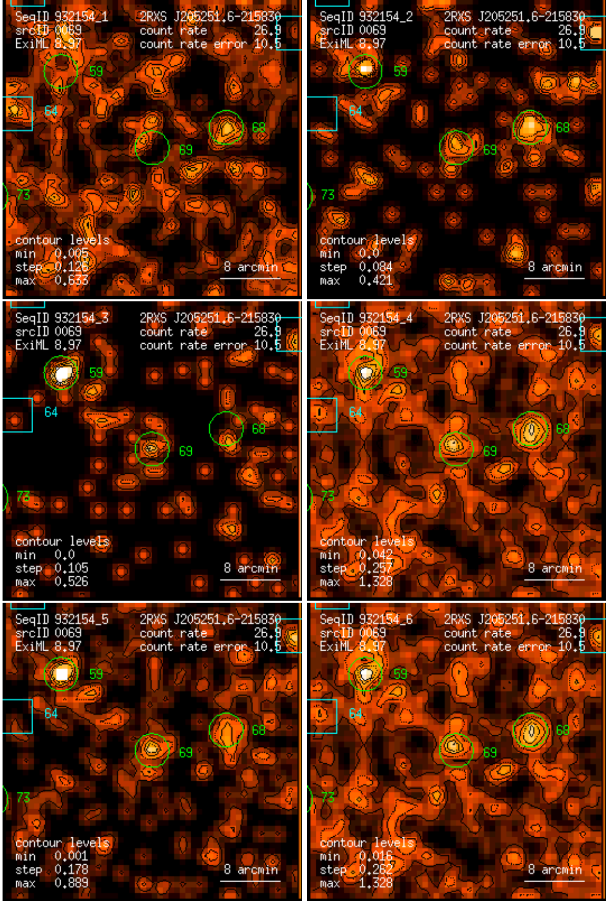
Figure 69: RASS 932154: detection 0069: band rate images, Gaussian filter: (1) PSPC channels 11 – 41, (2) 52 – 90, (3) 91 – 201, (4) 11 – 235, (5) 52 – 201, (6) 11 – 201. Broad band rates in counts/ks. Band rate contour levels in counts/ks/arcmin 2 .
