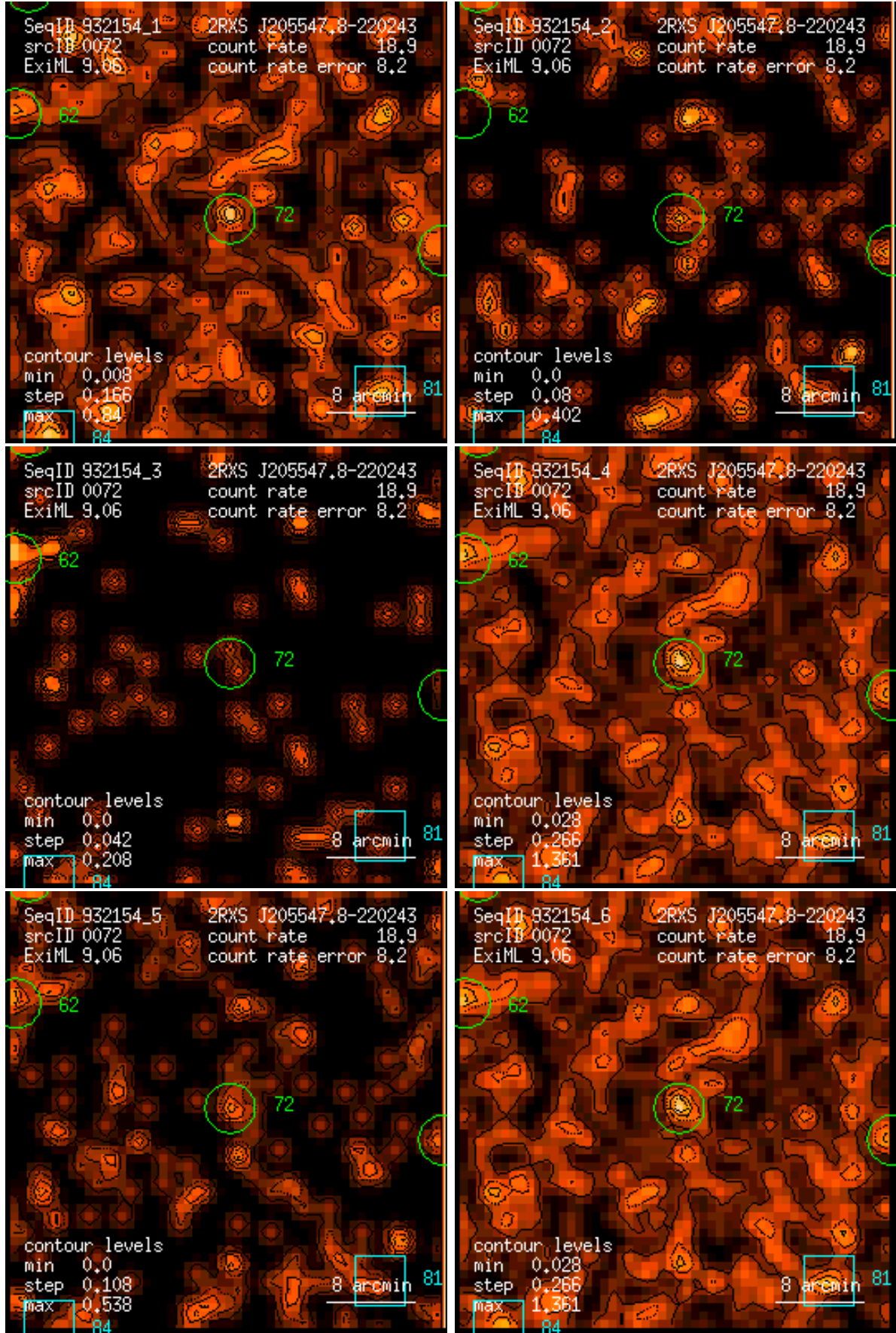
Figure 72: RASS 932154: detection 0072: band rate images, Gaussian filter: (1) PSPC channels 11 – 41, (2) 52 – 90, (3) 91 – 201, (4) 11 – 235, (5) 52 – 201, (6) 11 – 201. Broad band rates in counts/ks. Band rate contour levels in counts/ks/arcmin 2 .
