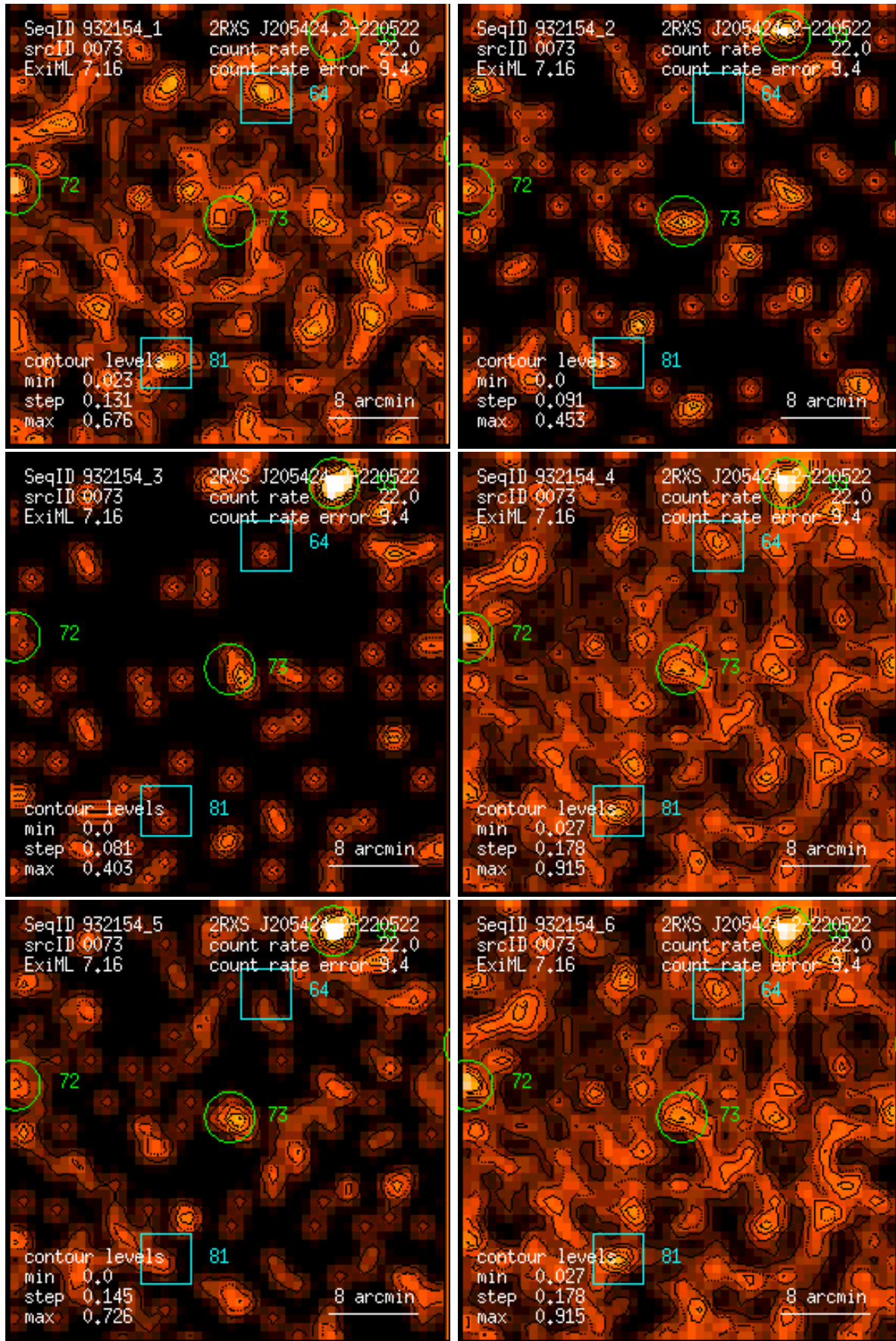
Figure 73: RASS 932154: detection 0073: band rate images, Gaussian filter: (1) PSPC channels 11 – 41, (2) 52 – 90, (3) 91 – 201, (4) 11 – 235, (5) 52 – 201, (6) 11 – 201. Broad band rates in counts/ks. Band rate contour levels in counts/ks/arcmin 2 .
