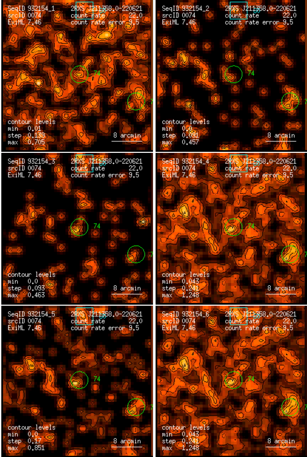
Figure 74: RASS 932154: detection 0074: band rate images, Gaussian filter: (1) PSPC channels 11 – 41, (2) 52 – 90, (3) 91 – 201, (4) 11 – 235, (5) 52 – 201, (6) 11 – 201. Broad band rates in counts/ks. Band rate contour levels in counts/ks/arcmin 2 .
