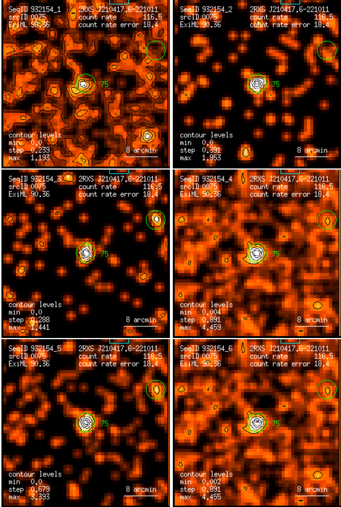
Figure 75: RASS 932154: detection 0075: band rate images, Gaussian filter: (1) PSPC channels 11 – 41, (2) 52 – 90, (3) 91 – 201, (4) 11 – 235, (5) 52 – 201, (6) 11 – 201. Broad band rates in counts/ks. Band rate contour levels in counts/ks/arcmin 2 .
