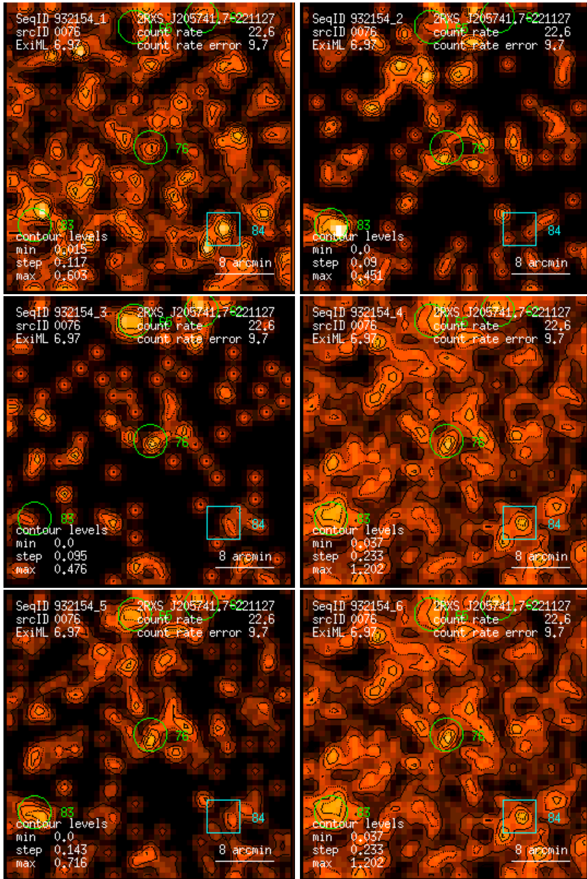
Figure 76: RASS 932154: detection 0076: band rate images, Gaussian filter: (1) PSPC channels 11 – 41, (2) 52 – 90, (3) 91 – 201, (4) 11 – 235, (5) 52 – 201, (6) 11 – 201. Broad band rates in counts/ks. Band rate contour levels in counts/ks/arcmin 2 .
