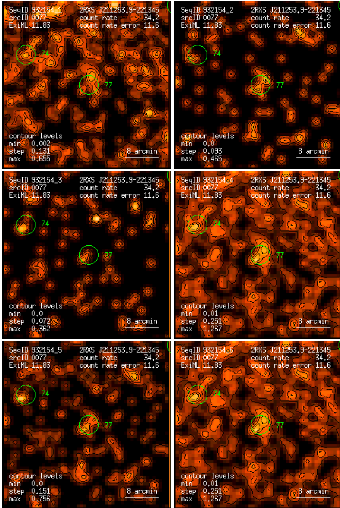
Figure 77: RASS 932154: detection 0077: band rate images, Gaussian filter: (1) PSPC channels 11 – 41, (2) 52 – 90, (3) 91 – 201, (4) 11 – 235, (5) 52 – 201, (6) 11 – 201. Broad band rates in counts/ks. Band rate contour levels in counts/ks/arcmin 2 .
