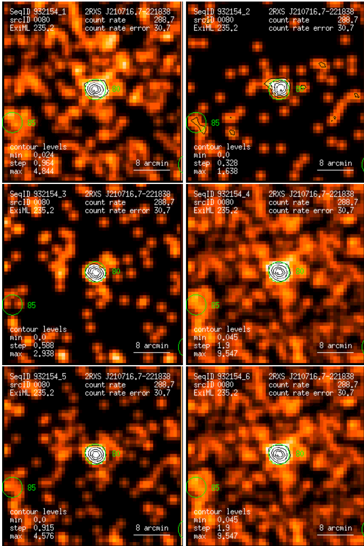
Figure 80: RASS 932154: detection 0080: band rate images, Gaussian filter: (1) PSPC channels 11 – 41, (2) 52 – 90, (3) 91 – 201, (4) 11 – 235, (5) 52 – 201, (6) 11 – 201. Broad band rates in counts/ks. Band rate contour levels in counts/ks/arcmin 2 .
