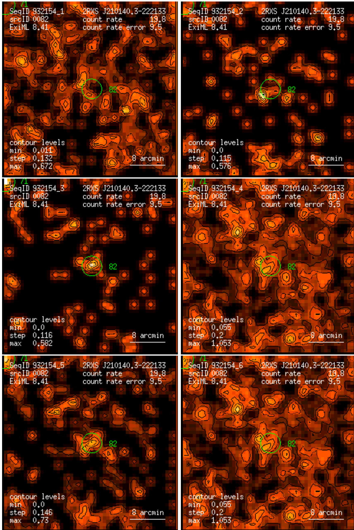
Figure 82: RASS 932154: detection 0082: band rate images, Gaussian filter: (1) PSPC channels 11 – 41, (2) 52 – 90, (3) 91 – 201, (4) 11 – 235, (5) 52 – 201, (6) 11 – 201. Broad band rates in counts/ks. Band rate contour levels in counts/ks/arcmin 2 .
