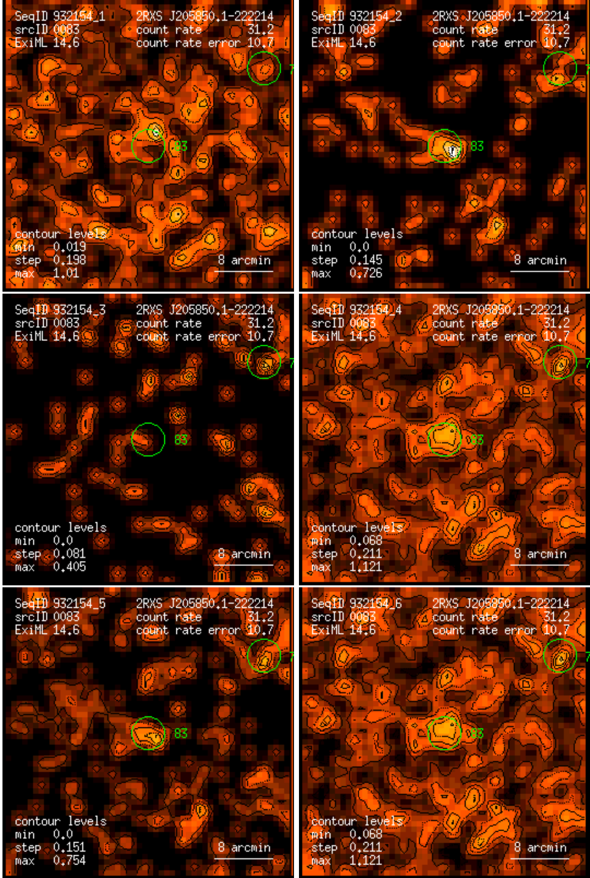
Figure 83: RASS 932154: detection 0083: band rate images, Gaussian filter: (1) PSPC channels 11 – 41, (2) 52 – 90, (3) 91 – 201, (4) 11 – 235, (5) 52 – 201, (6) 11 – 201. Broad band rates in counts/ks. Band rate contour levels in counts/ks/arcmin 2 .
