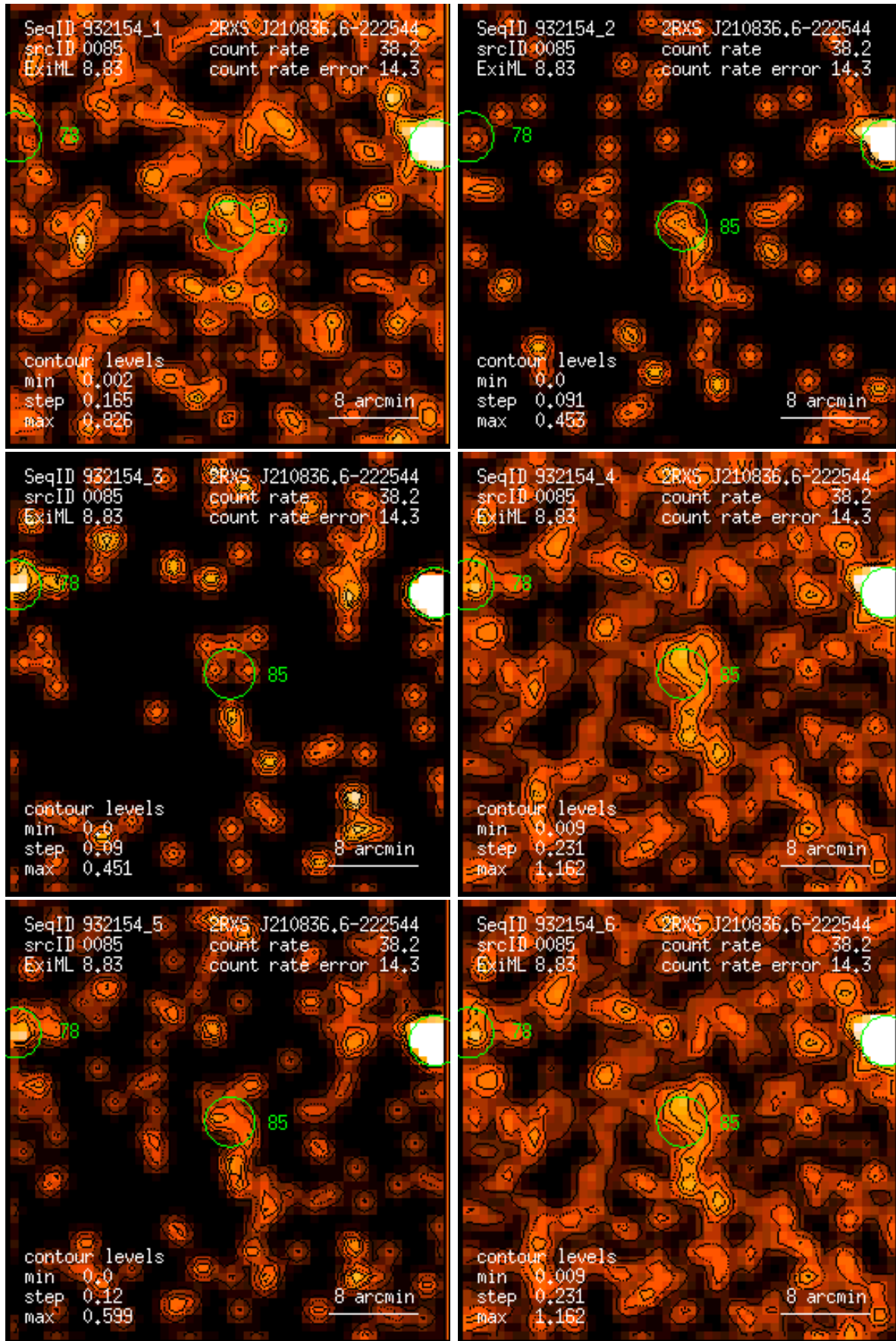
Figure 85: RASS 932154: detection 0085: band rate images, Gaussian filter: (1) PSPC channels 11 – 41, (2) 52 – 90, (3) 91 – 201, (4) 11 – 235, (5) 52 – 201, (6) 11 – 201. Broad band rates in counts/ks. Band rate contour levels in counts/ks/arcmin 2 .
