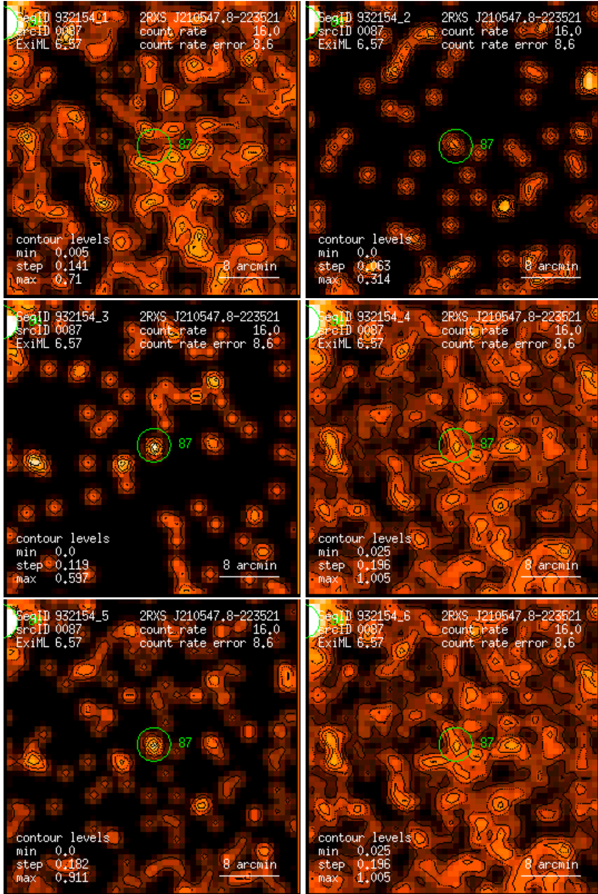
Figure 87: RASS 932154: detection 0087: band rate images, Gaussian filter: (1) PSPC channels 11 – 41, (2) 52 – 90, (3) 91 – 201, (4) 11 – 235, (5) 52 – 201, (6) 11 – 201. Broad band rates in counts/ks. Band rate contour levels in counts/ks/arcmin 2 .
