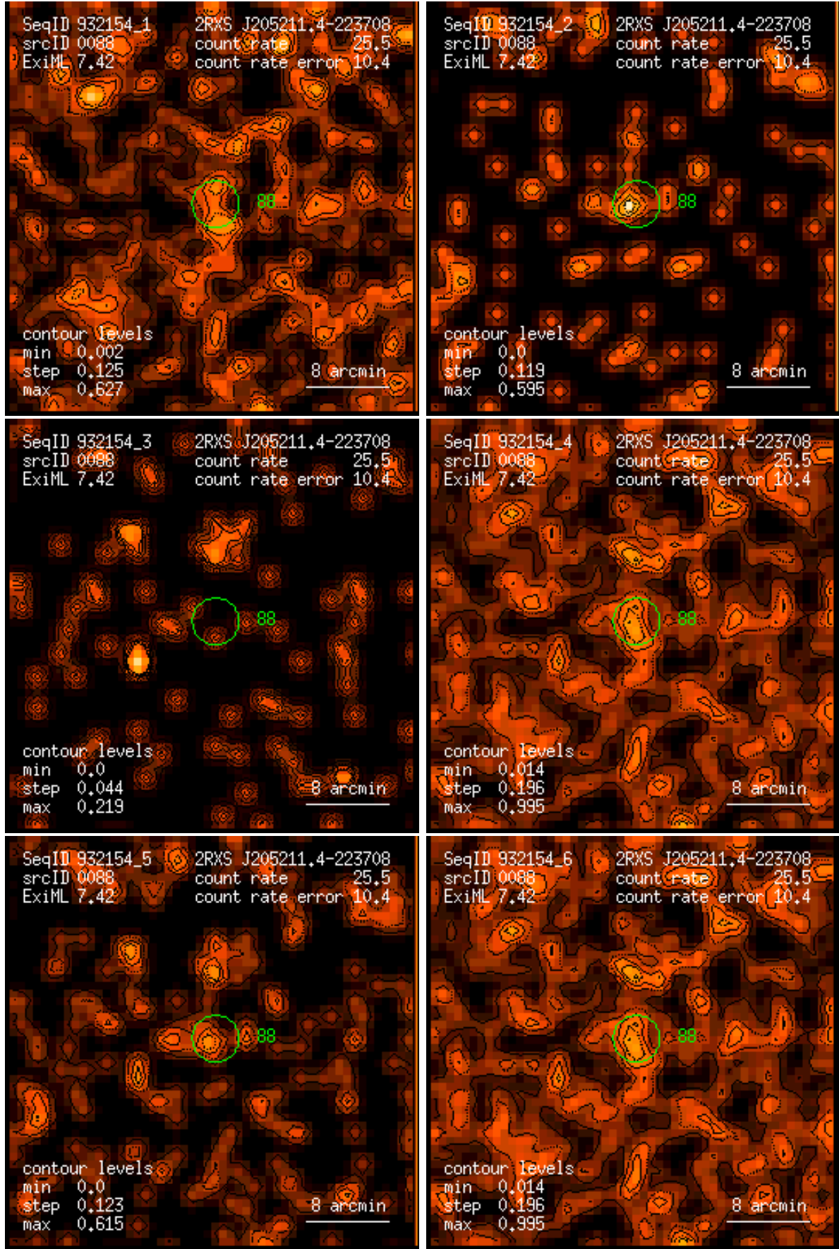
Figure 88: RASS 932154: detection 0088: band rate images, Gaussian filter: (1) PSPC channels 11 – 41, (2) 52 – 90, (3) 91 – 201, (4) 11 – 235, (5) 52 – 201, (6) 11 – 201. Broad band rates in counts/ks. Band rate contour levels in counts/ks/arcmin 2 .
