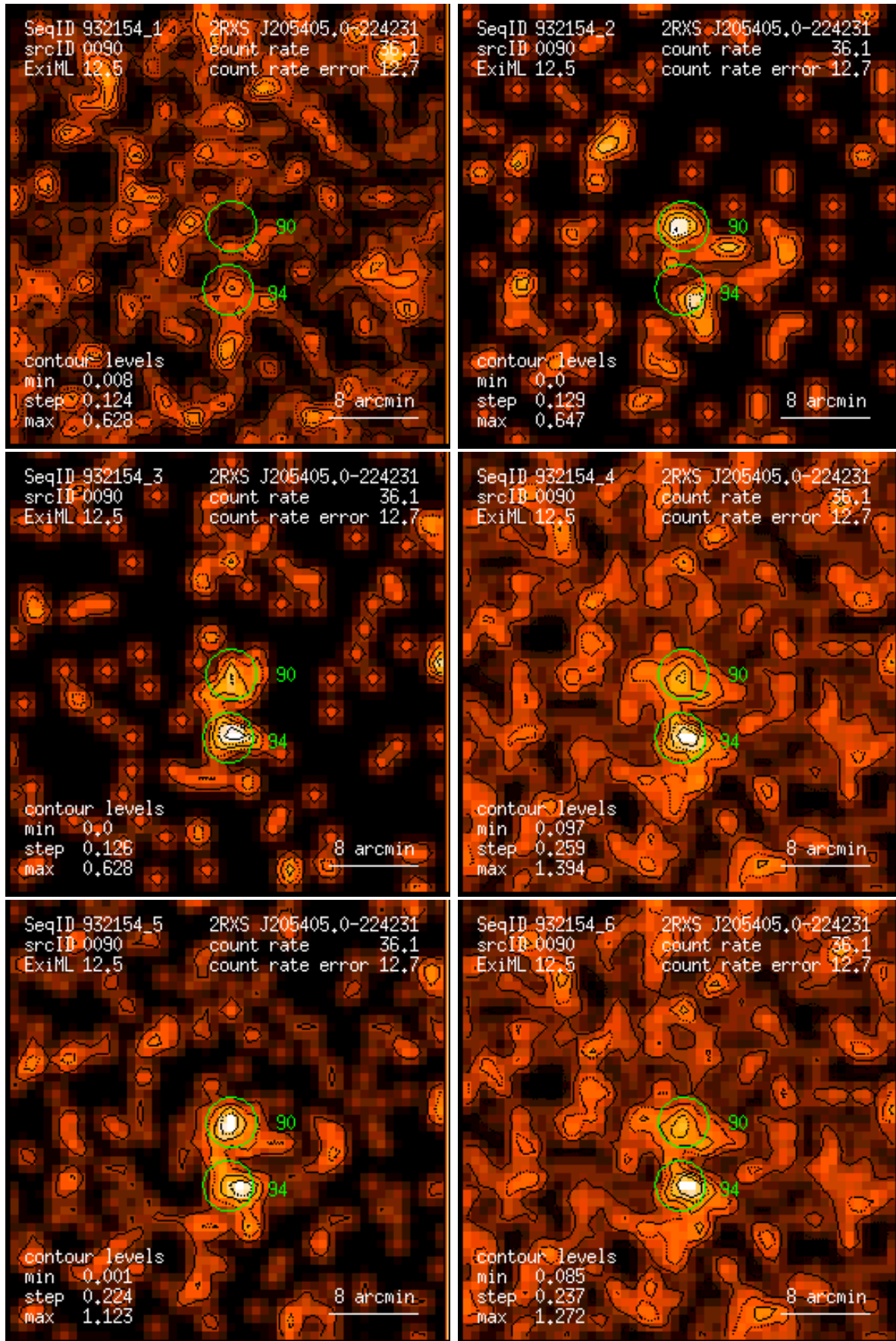
Figure 90: RASS 932154: detection 0090: band rate images, Gaussian filter: (1) PSPC channels 11 – 41, (2) 52 – 90, (3) 91 – 201, (4) 11 – 235, (5) 52 – 201, (6) 11 – 201. Broad band rates in counts/ks. Band rate contour levels in counts/ks/arcmin 2 .
