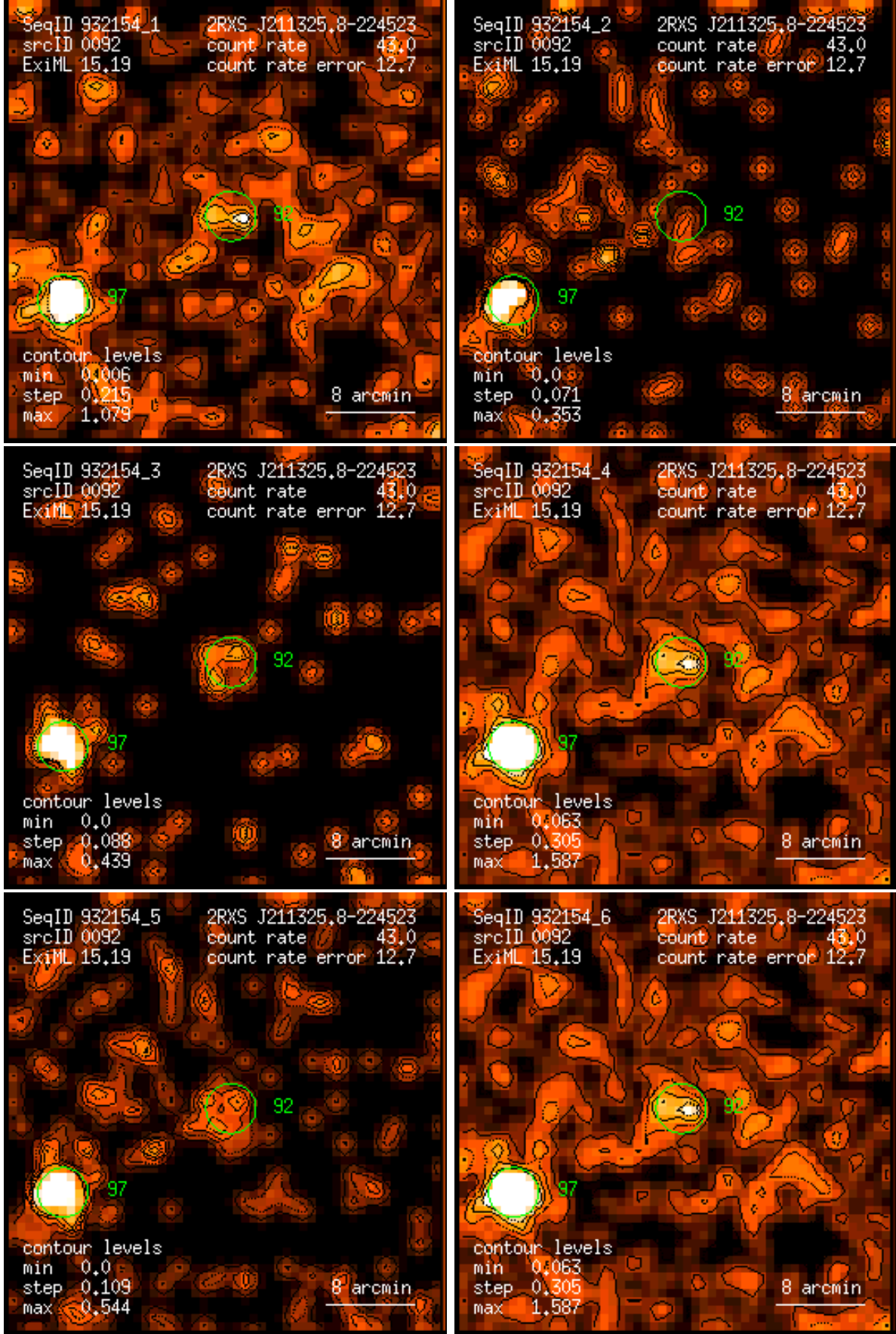
Figure 92: RASS 932154: detection 0092: band rate images, Gaussian filter: (1) PSPC channels 11 – 41, (2) 52 – 90, (3) 91 – 201, (4) 11 – 235, (5) 52 – 201, (6) 11 – 201. Broad band rates in counts/ks. Band rate contour levels in counts/ks/arcmin 2 .
